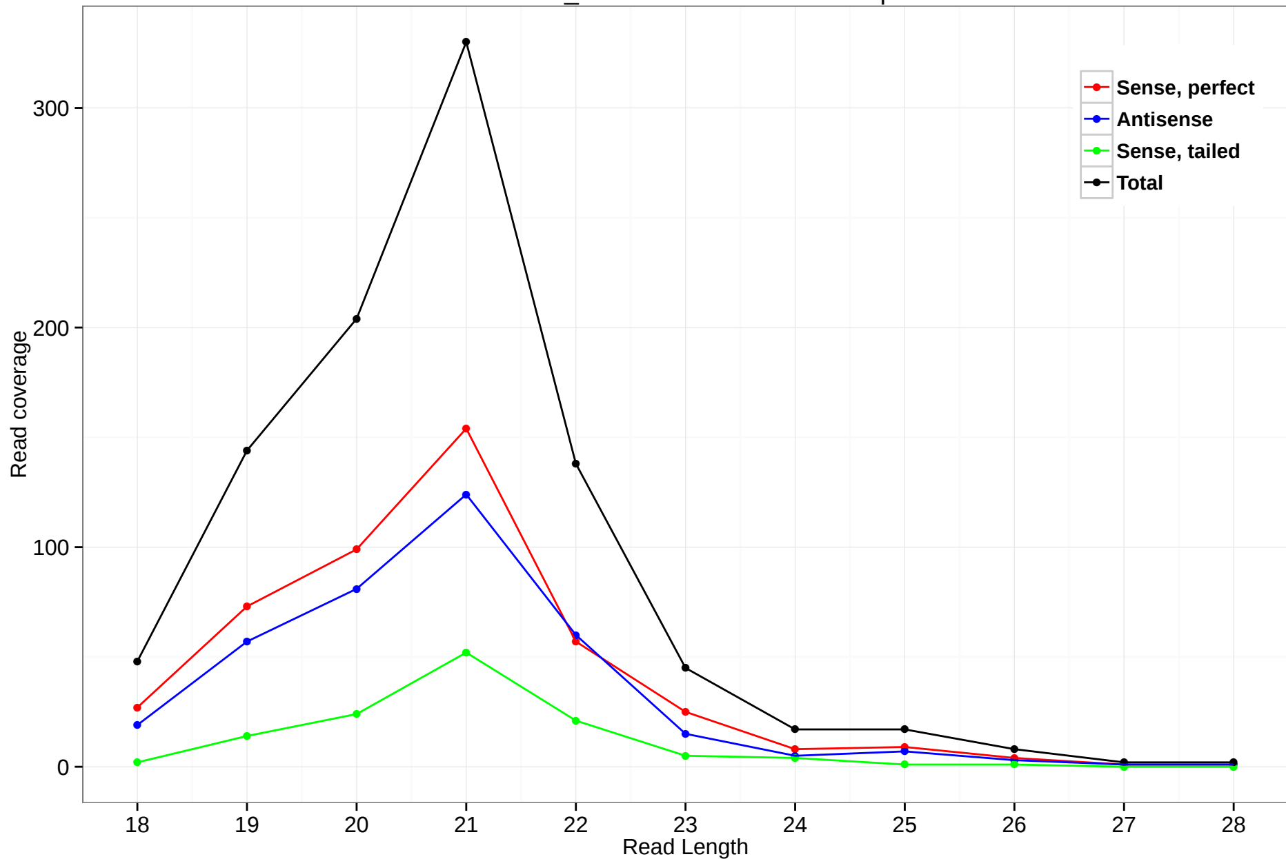
scaffold_4512:1280295-1283355.5p
