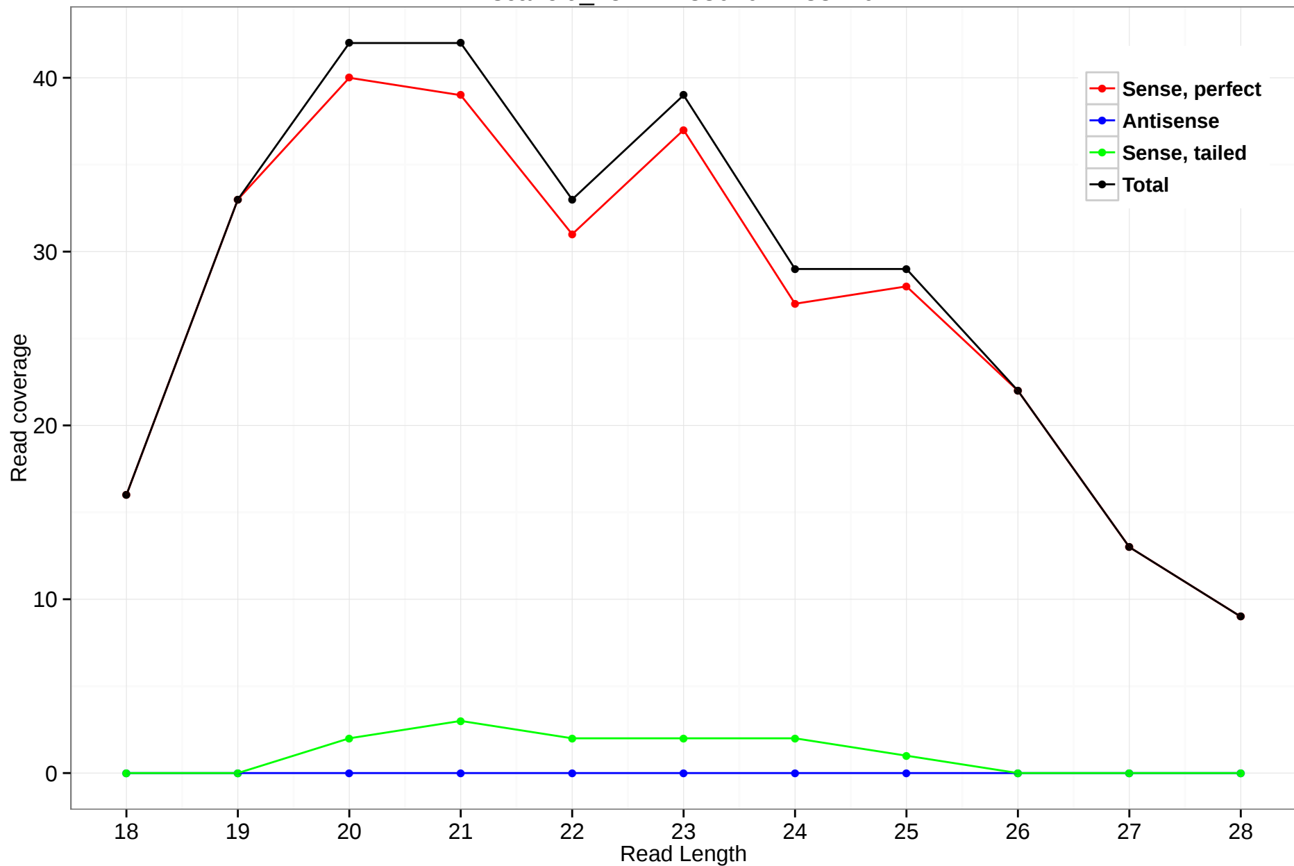
scaffold_4512:1233070-1233240
