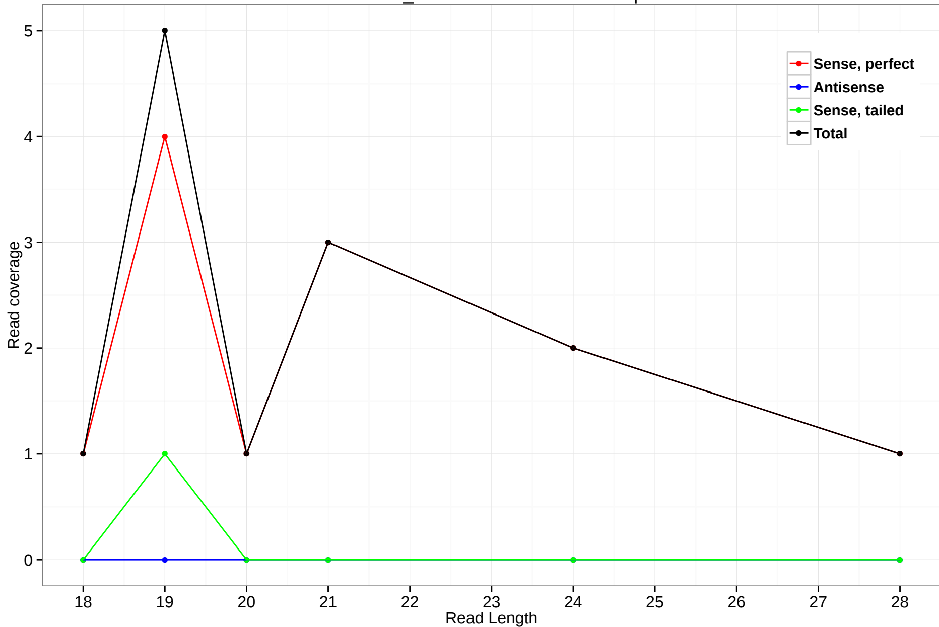
scaffold_4512:1215560-1216917.5p
