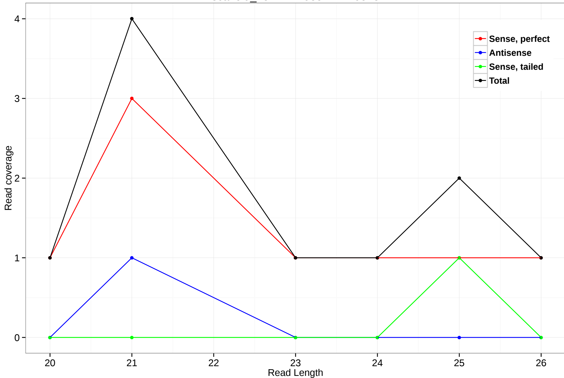
scaffold_4512:1179352-1179513
