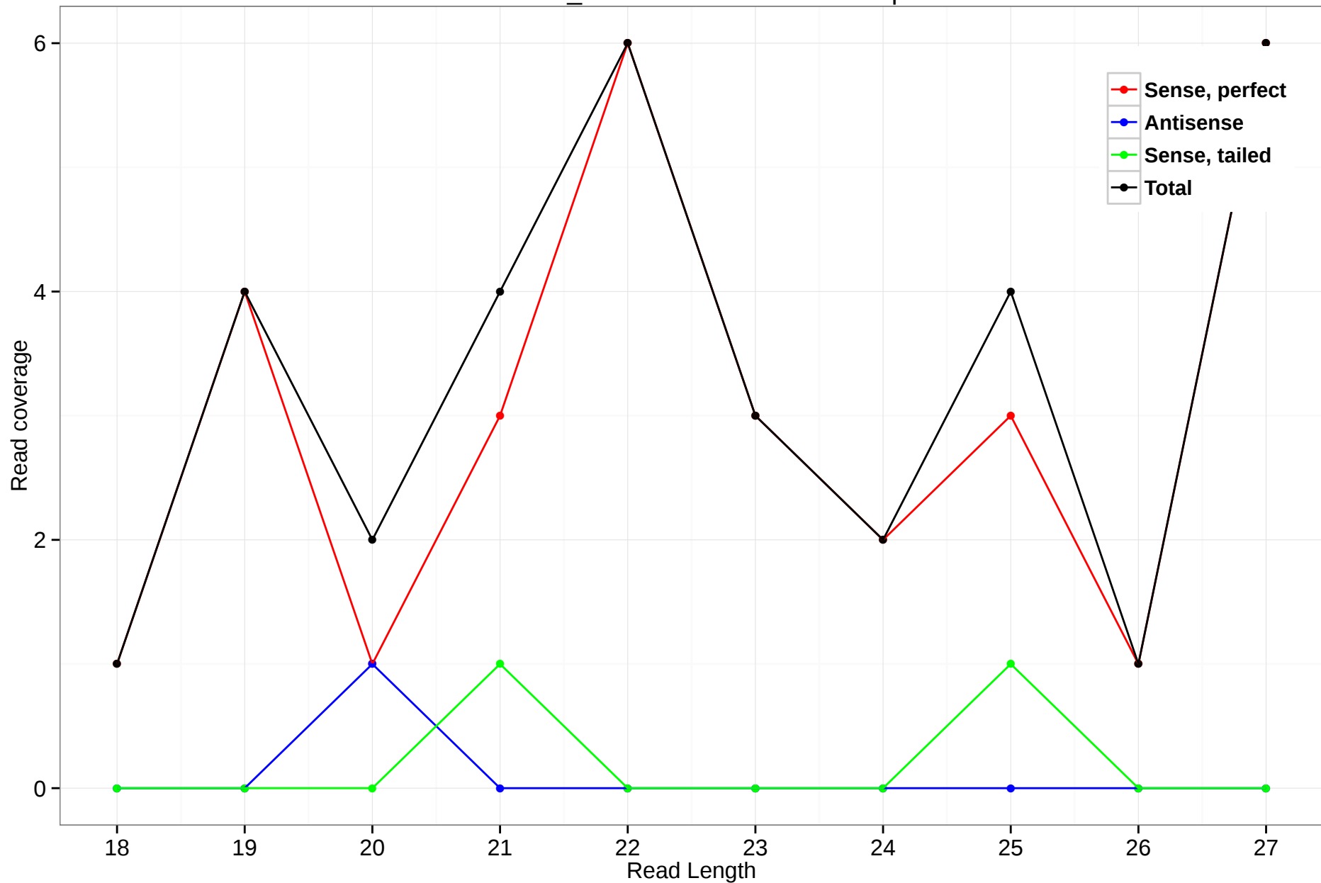
scaffold_4512:1169124-1170167.3p
