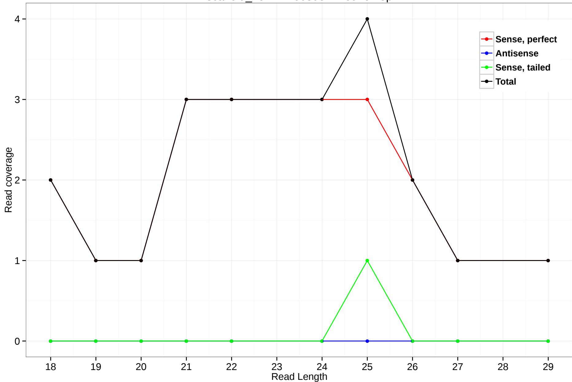
scaffold_4512:1166895-1169137.3p
