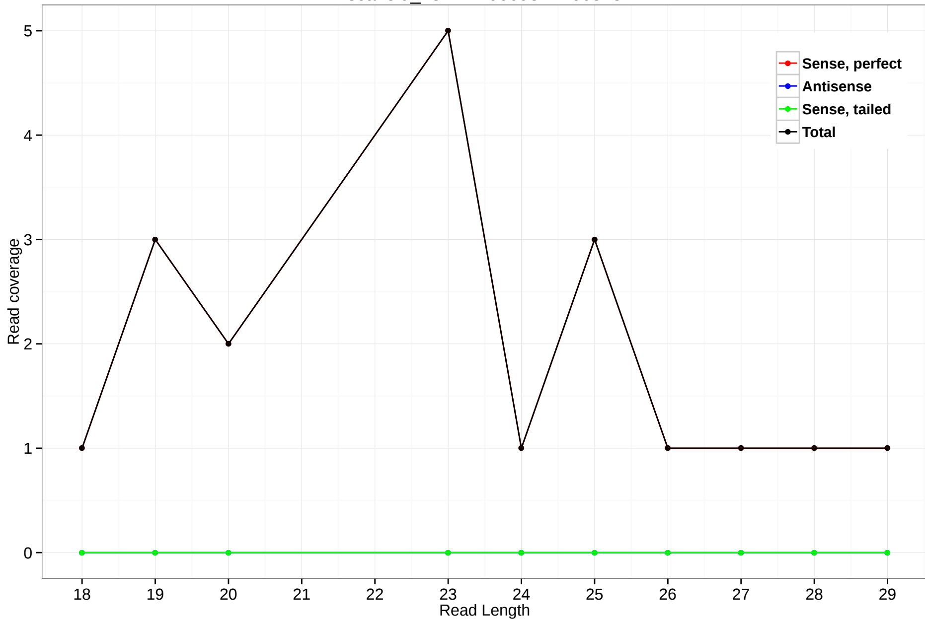
scaffold_4512:1166698-1166875
