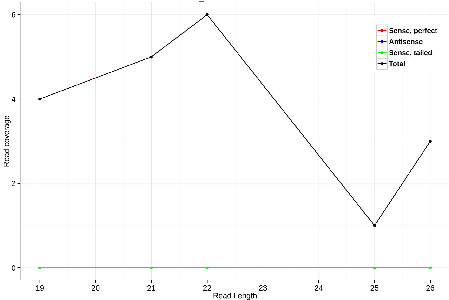
scaffold_4512:1088922-1089098
