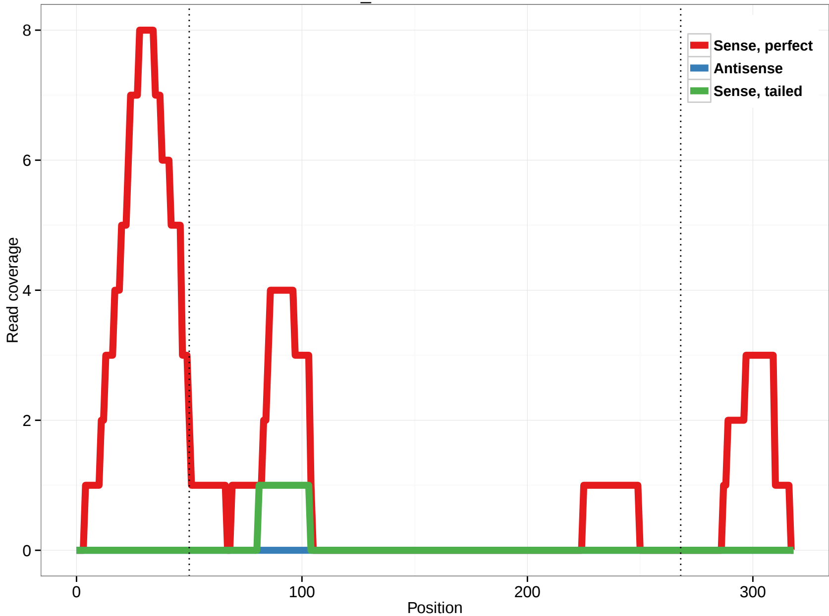
scaffold_4929:5409096-5409414
