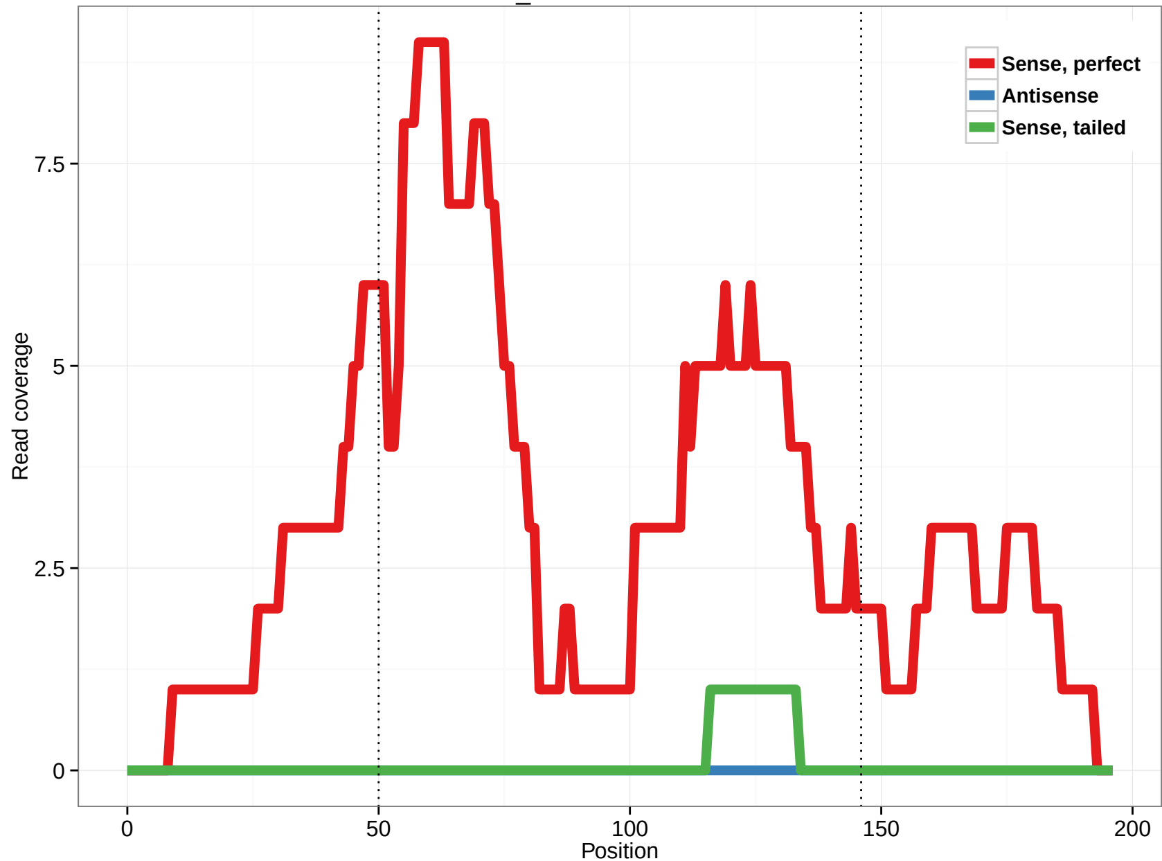
scaffold_4929:5125968-5126164
