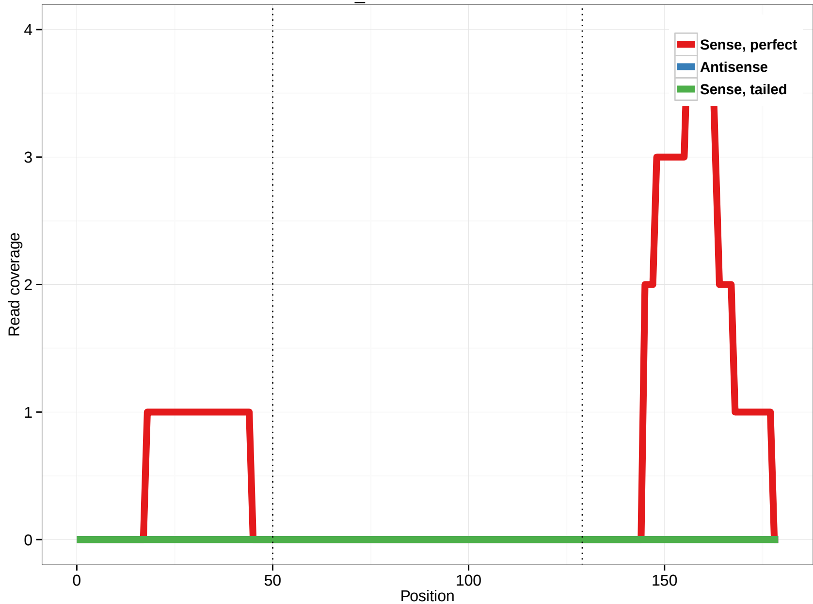
scaffold_4929:4910684-4910863
