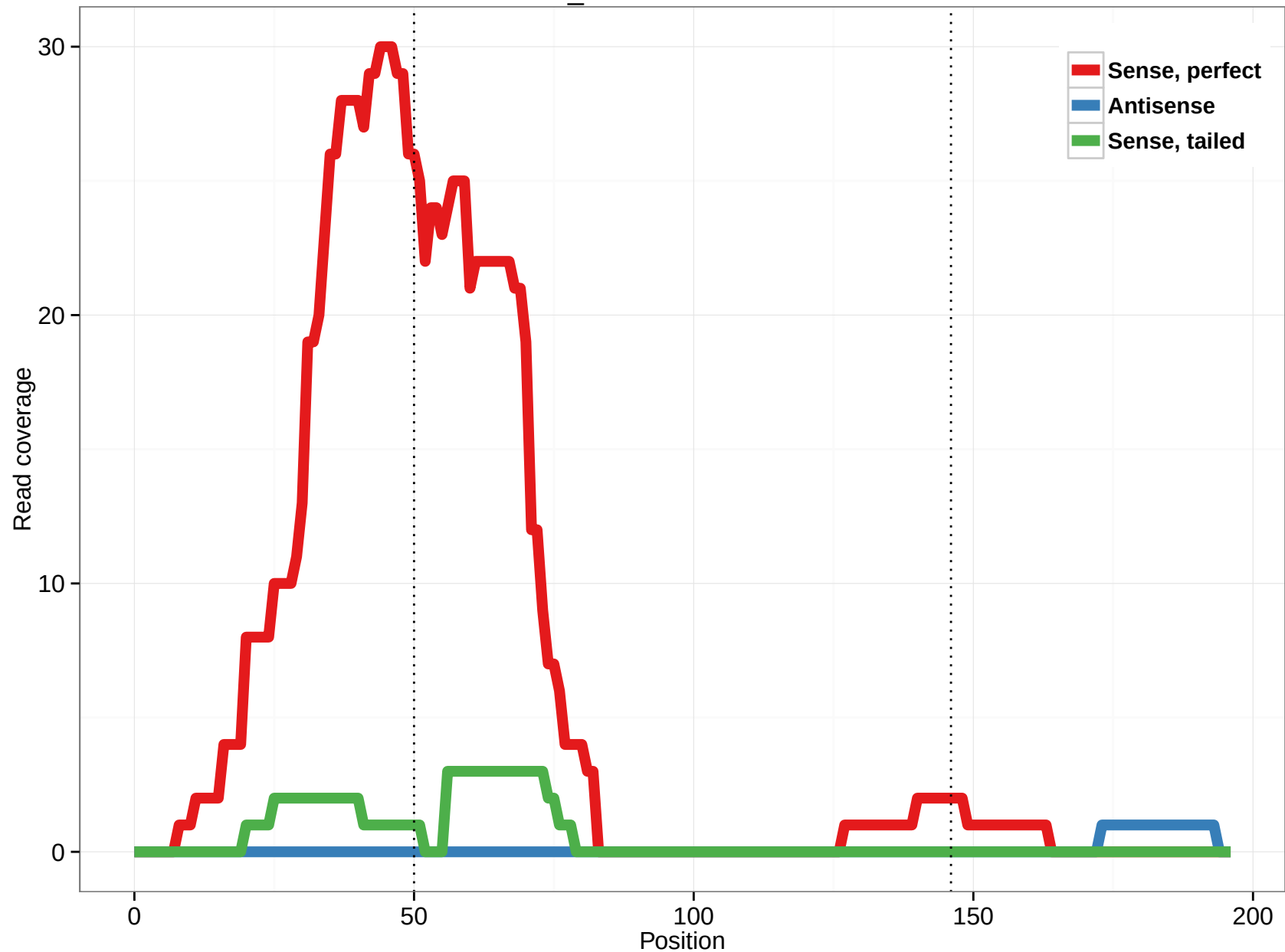
scaffold_4929:2903420-2903616
