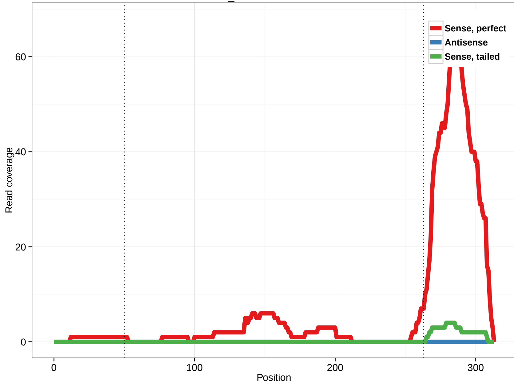
scaffold_4929:2413152-2413465
