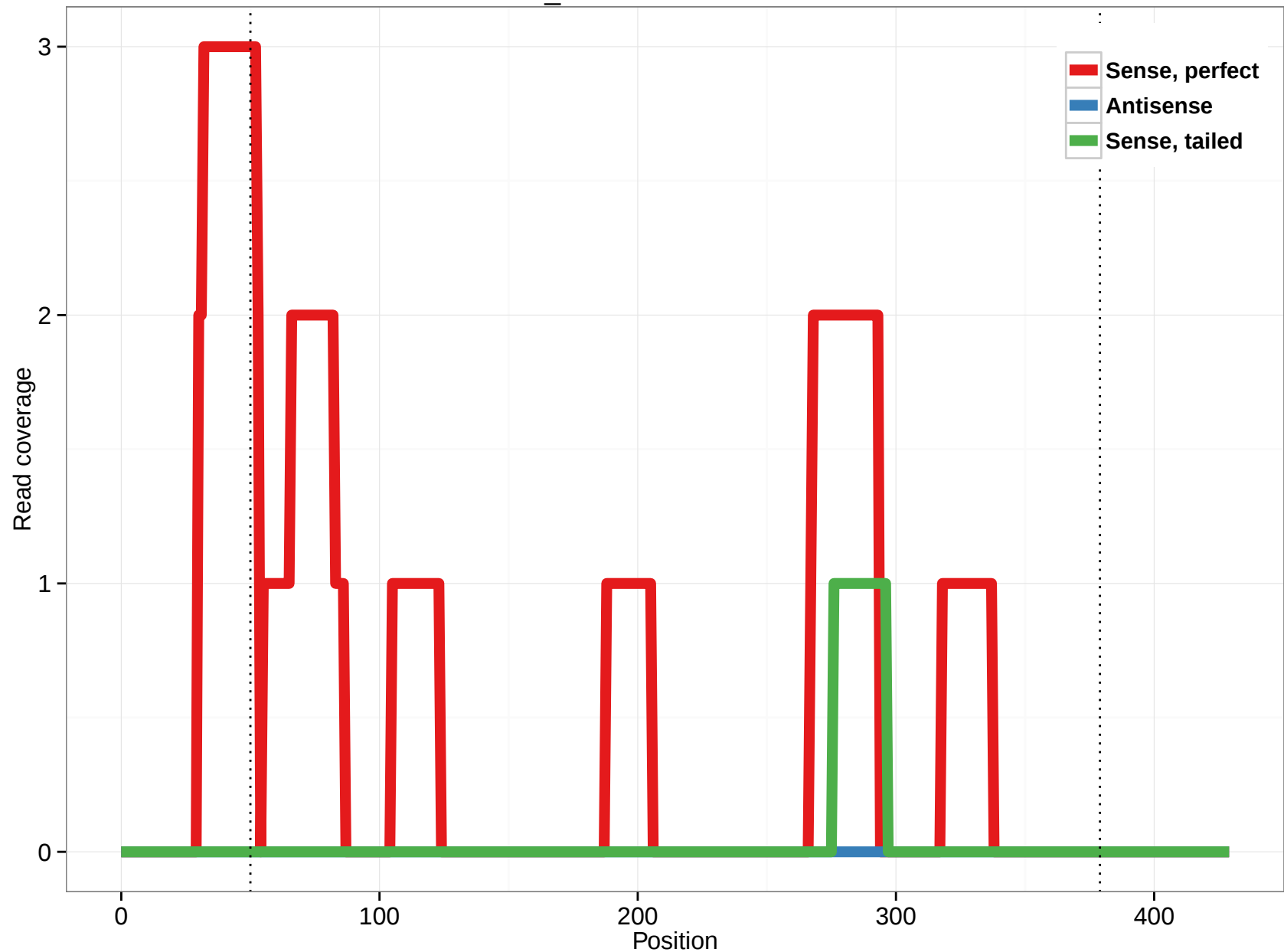
scaffold_4929:21290676-21291105
