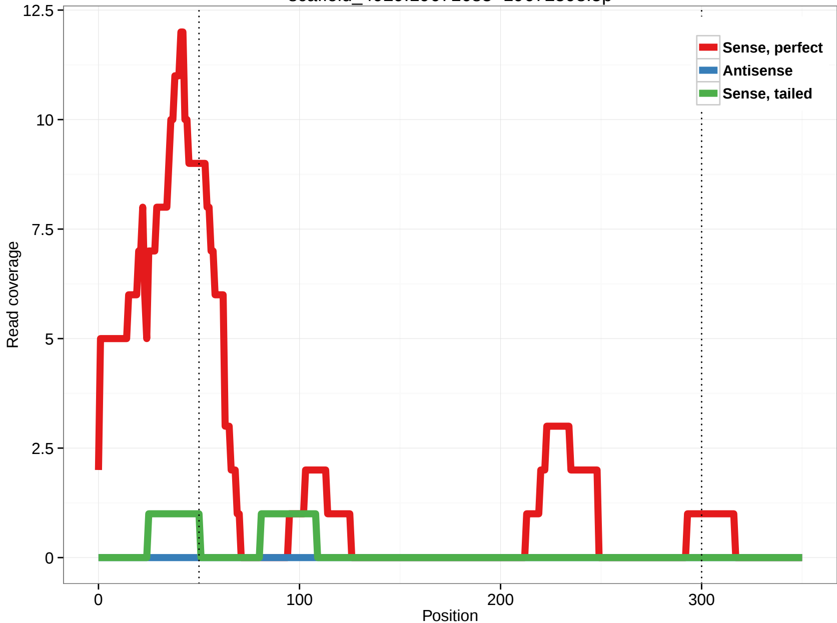
scaffold_4929:19671683-19672598.5p
