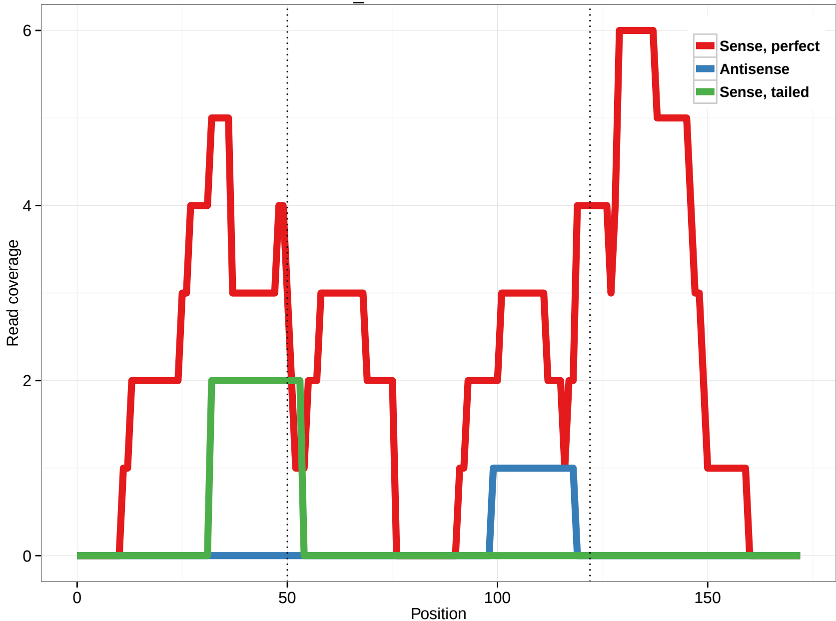
scaffold_4929:14738334-14738506
