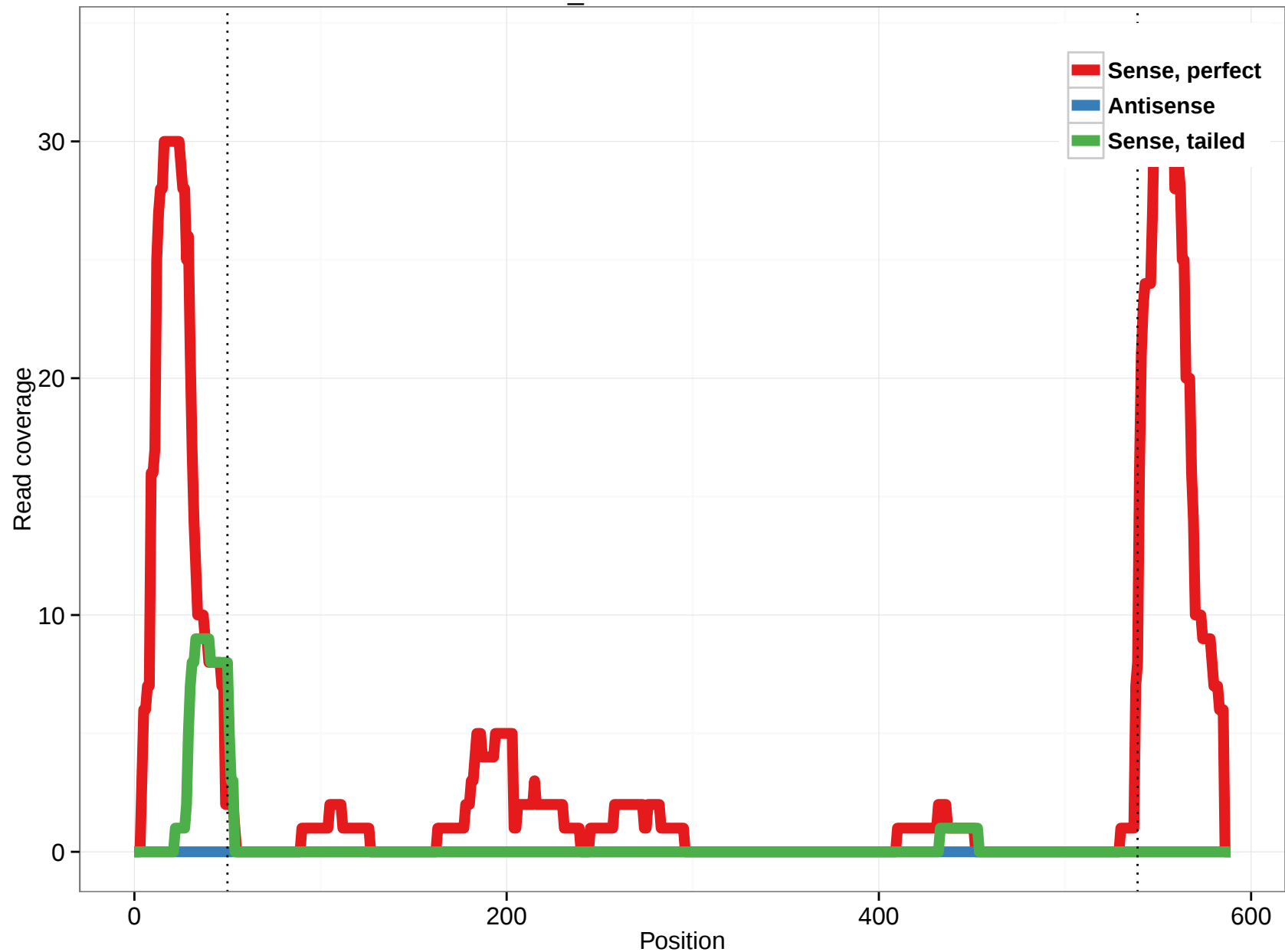
scaffold_4929:1404933-1405522
