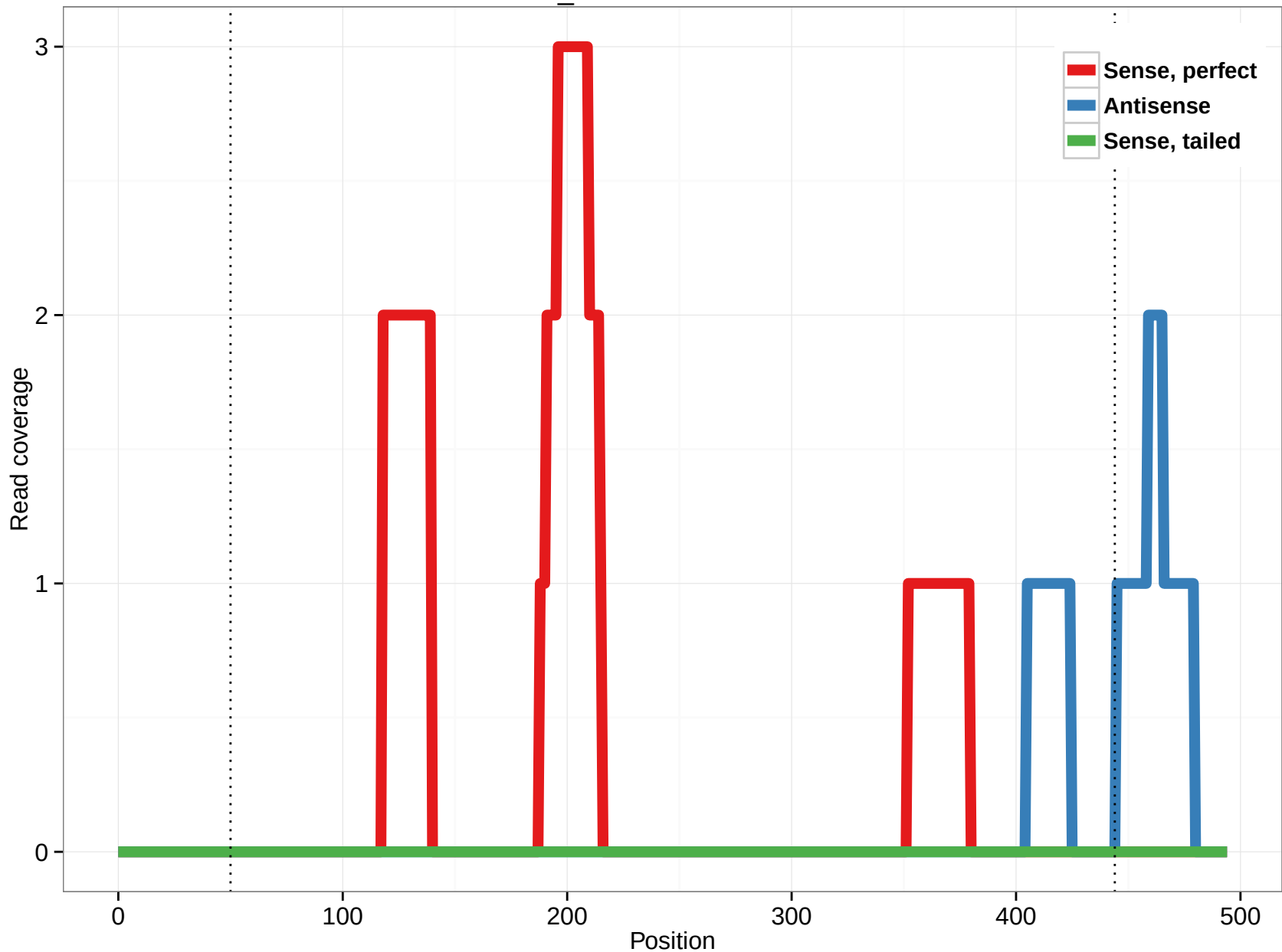
scaffold_4845:9580646-9581140
