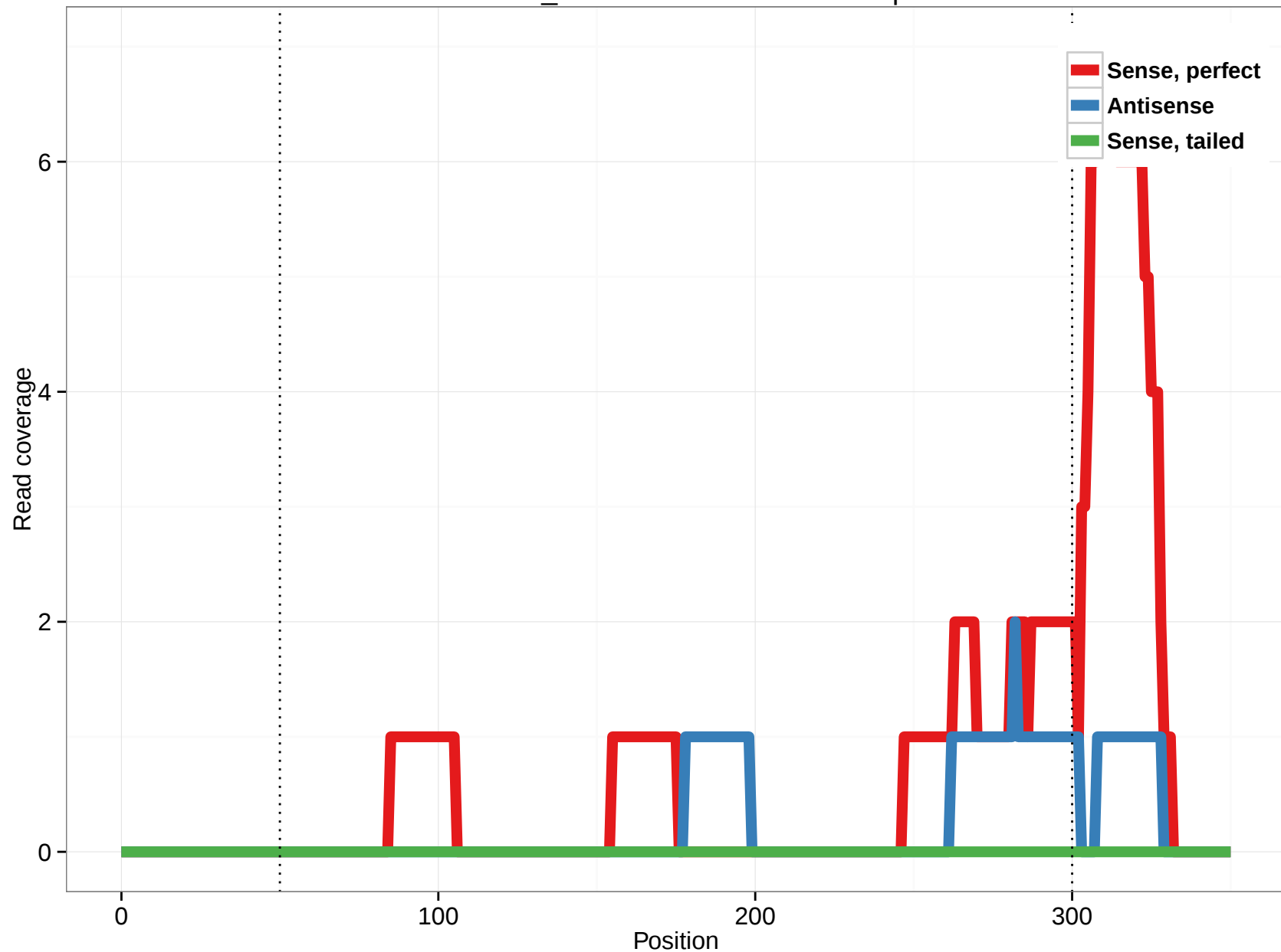
scaffold_4845:9548513-9550459.5p
