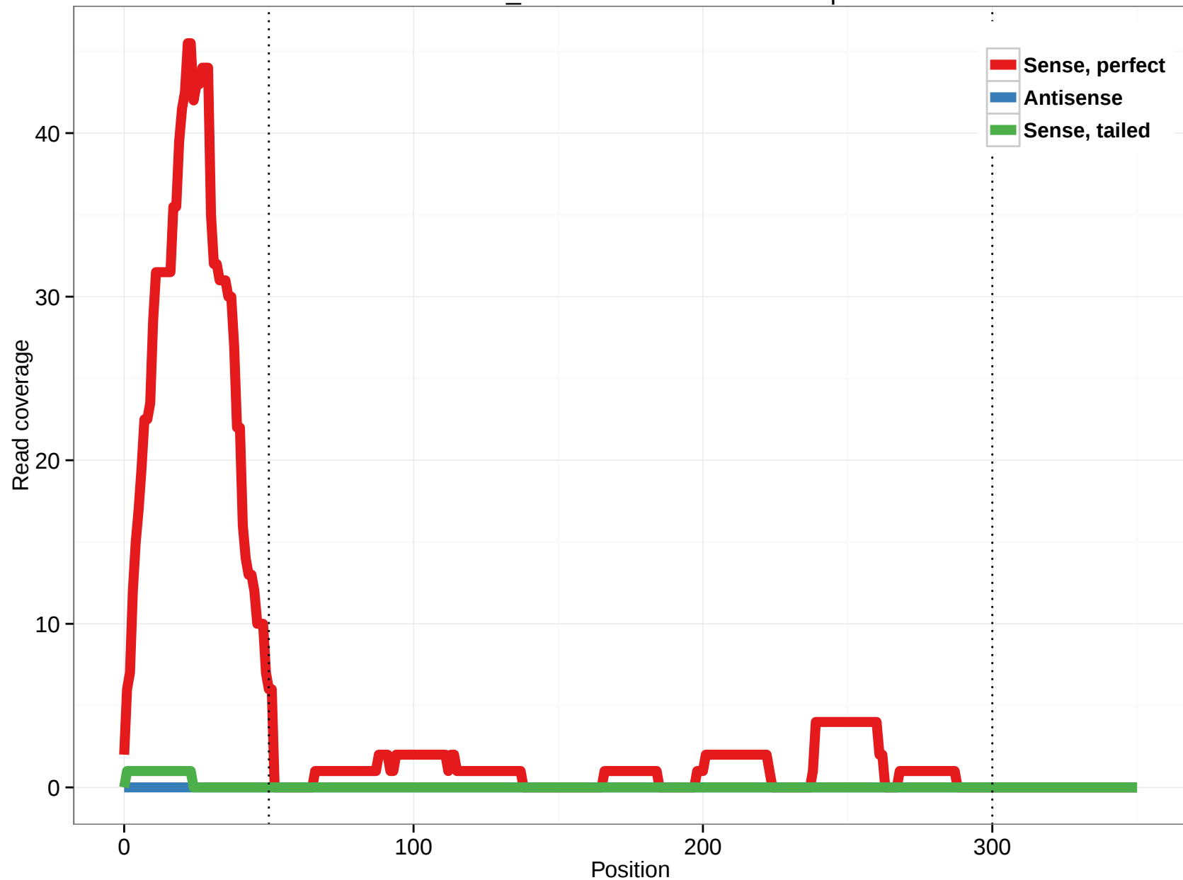
scaffold_4845:7698566-7699235.5p
