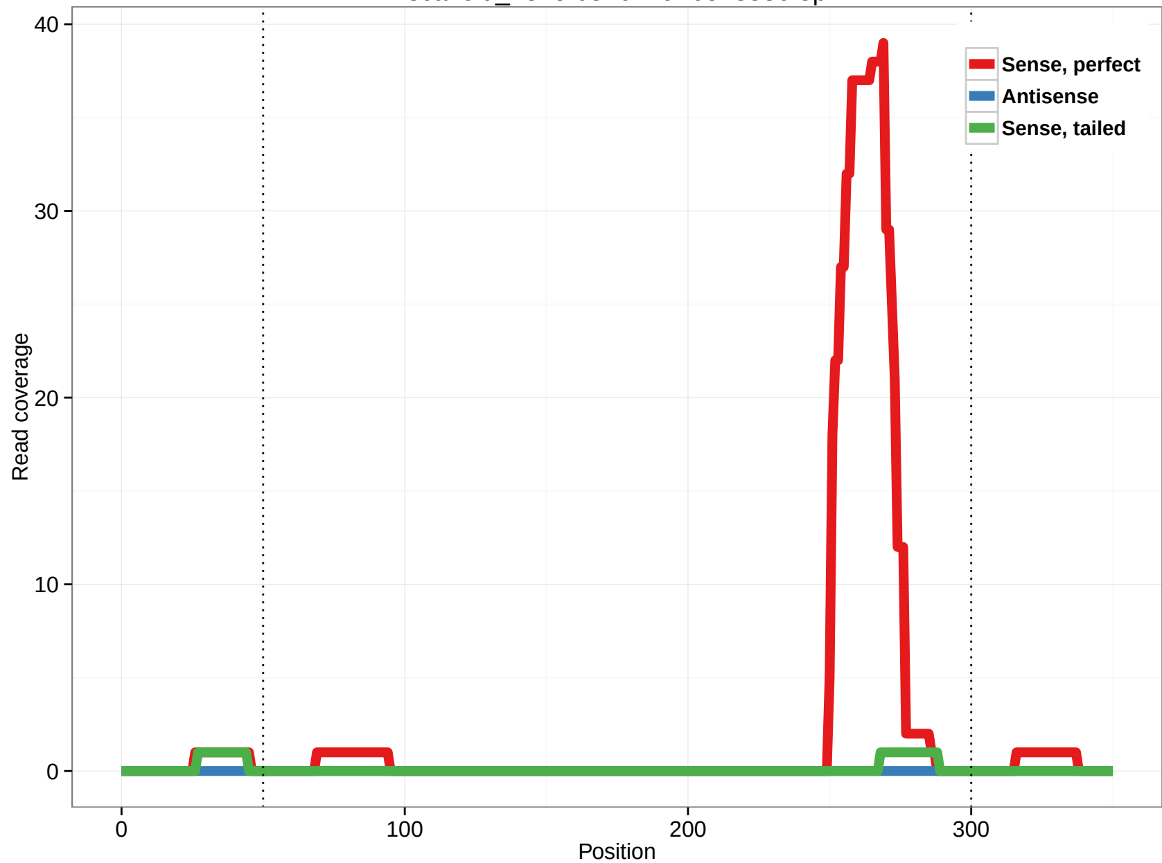
scaffold_4845:6846279-6848580.5p
