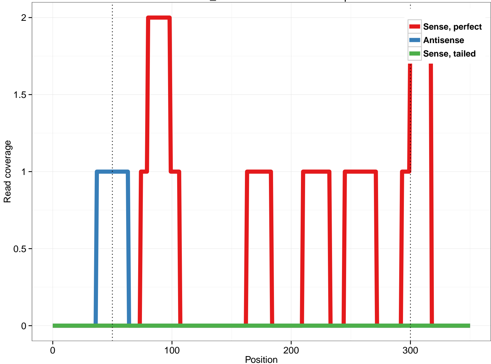
scaffold_4845:5298003-5299087.3p
