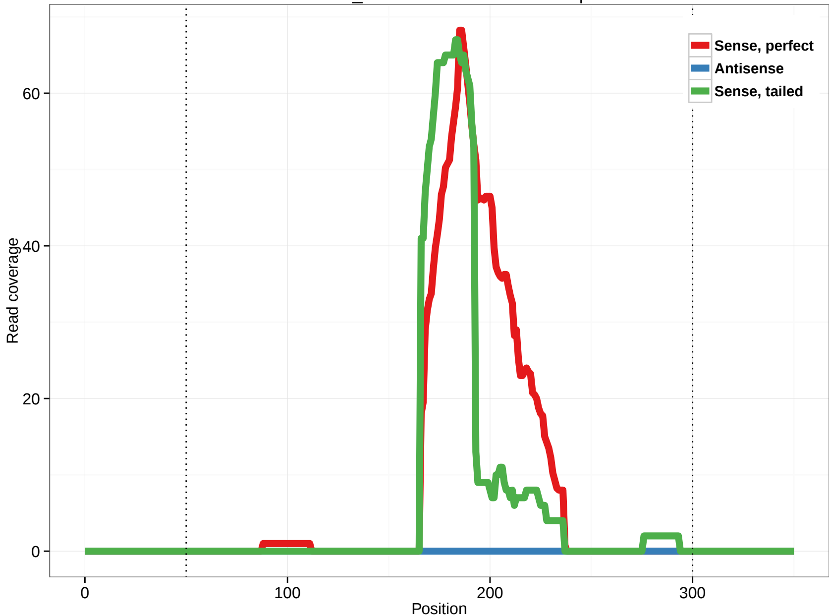
scaffold_4845:3811515-3812253.3p
