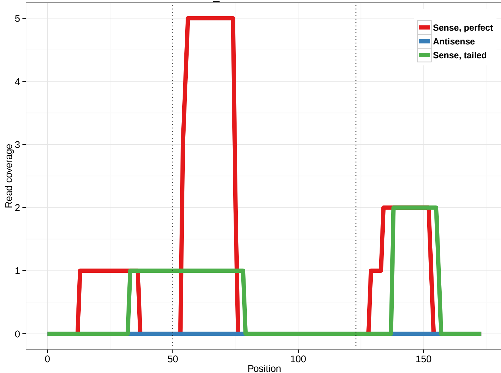
scaffold_4845:20924806-20924979
