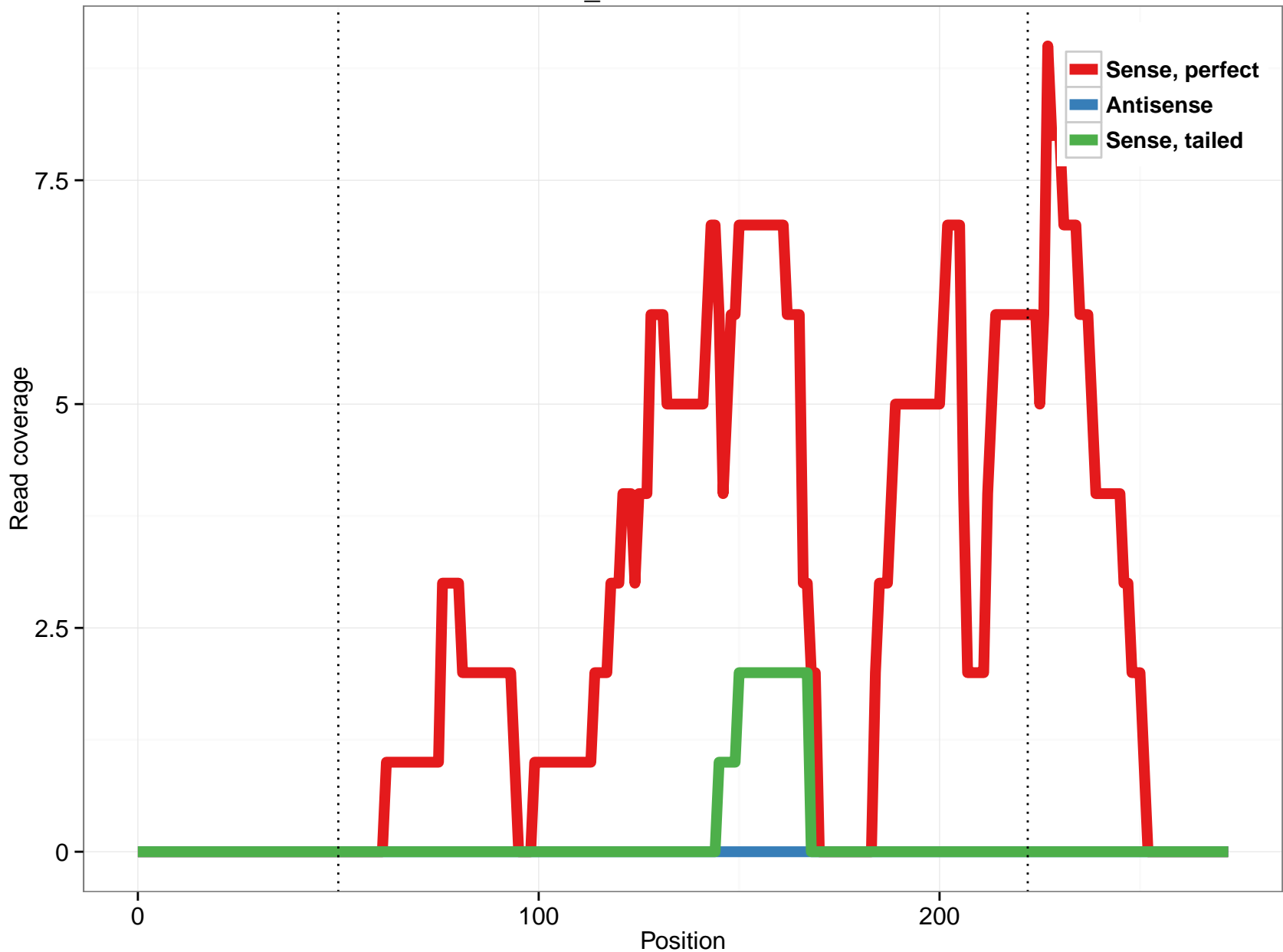
scaffold_4845:175569-175841
