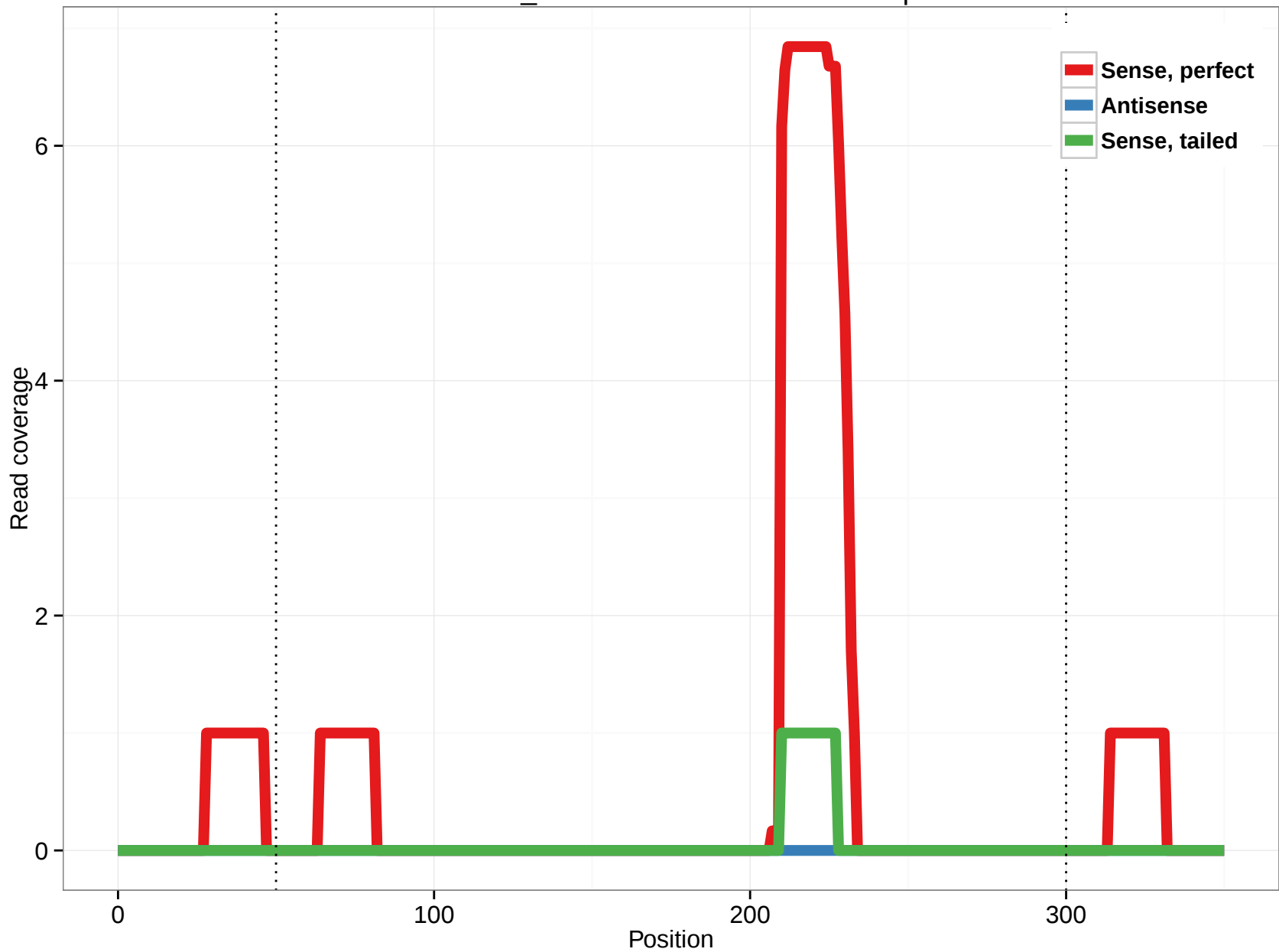
scaffold_4845:16425711-16426517.5p
