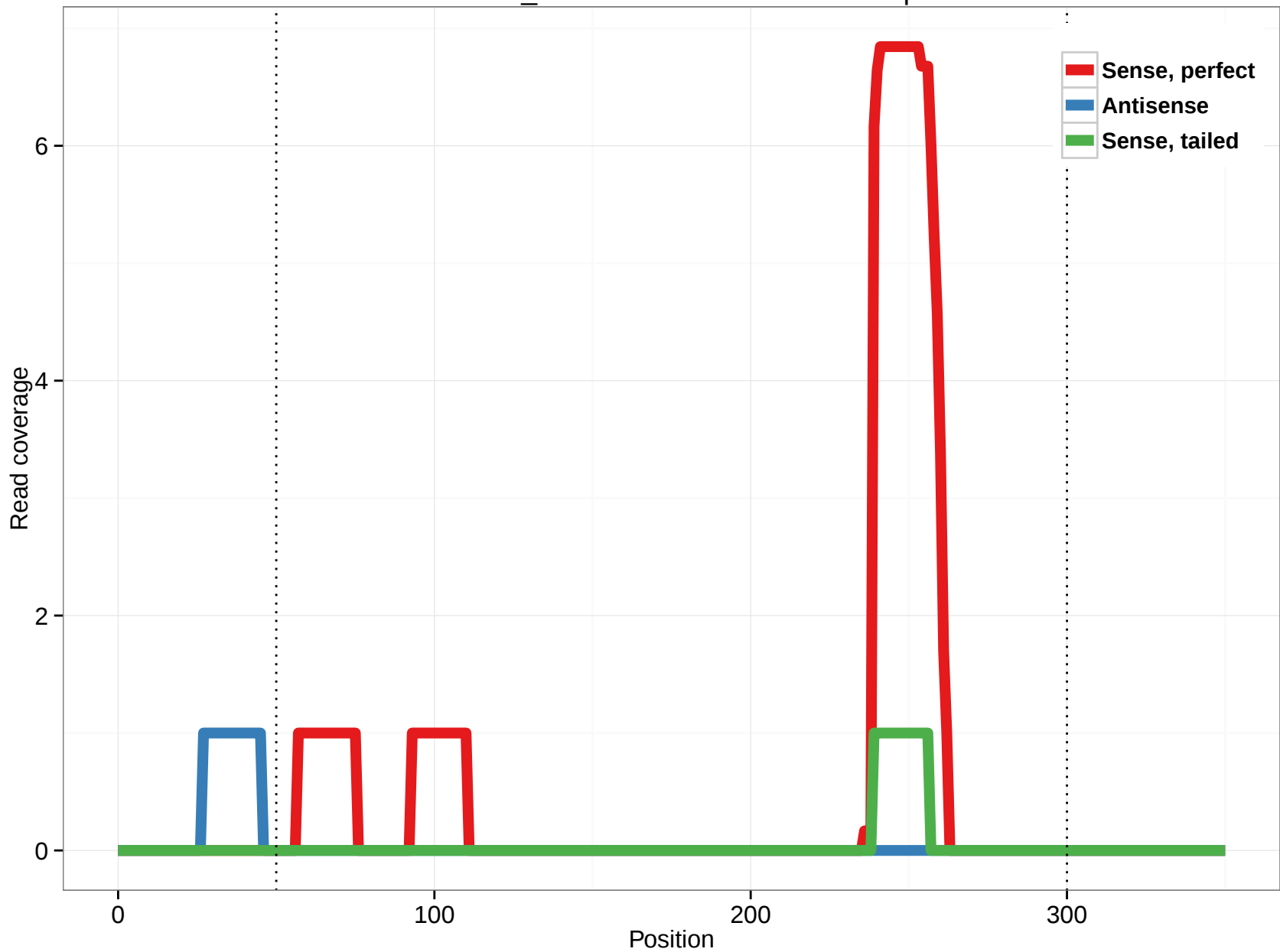
scaffold_4845:16425682-16426517.5p
