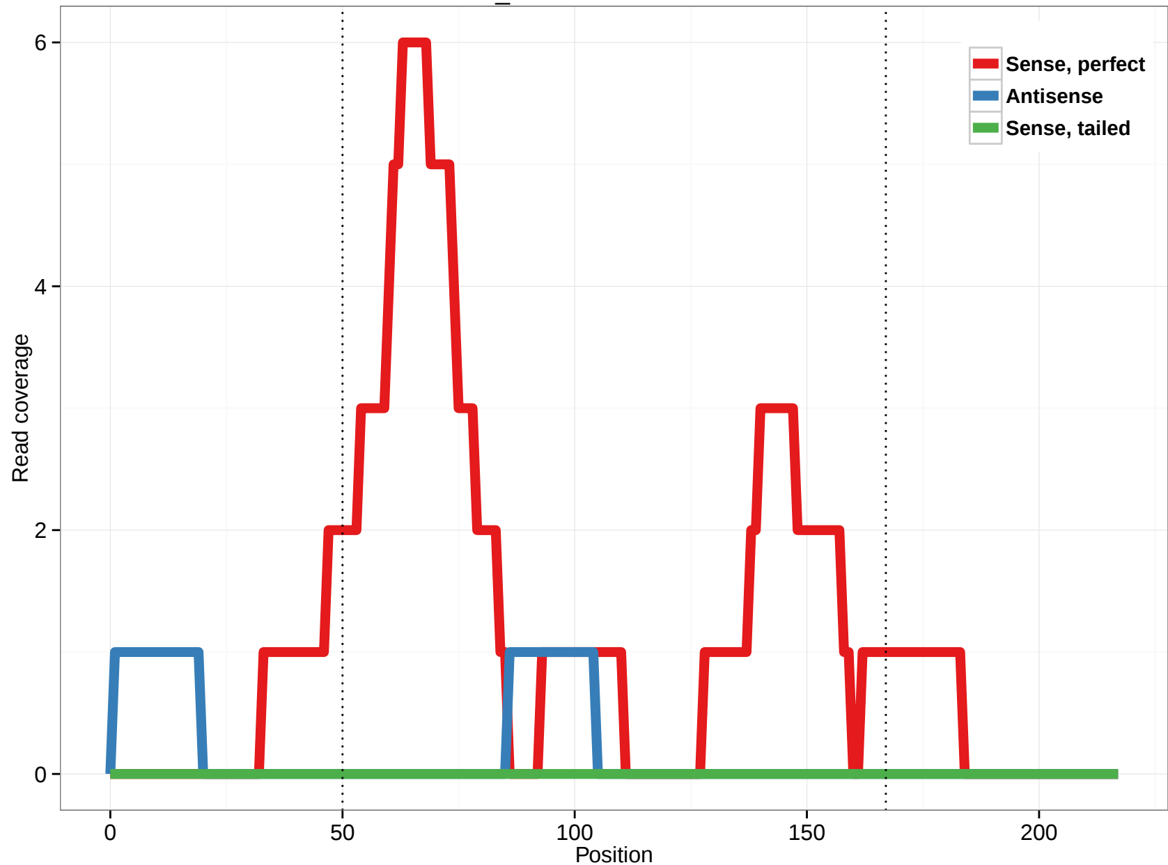
scaffold_4845:15693081-15693298
