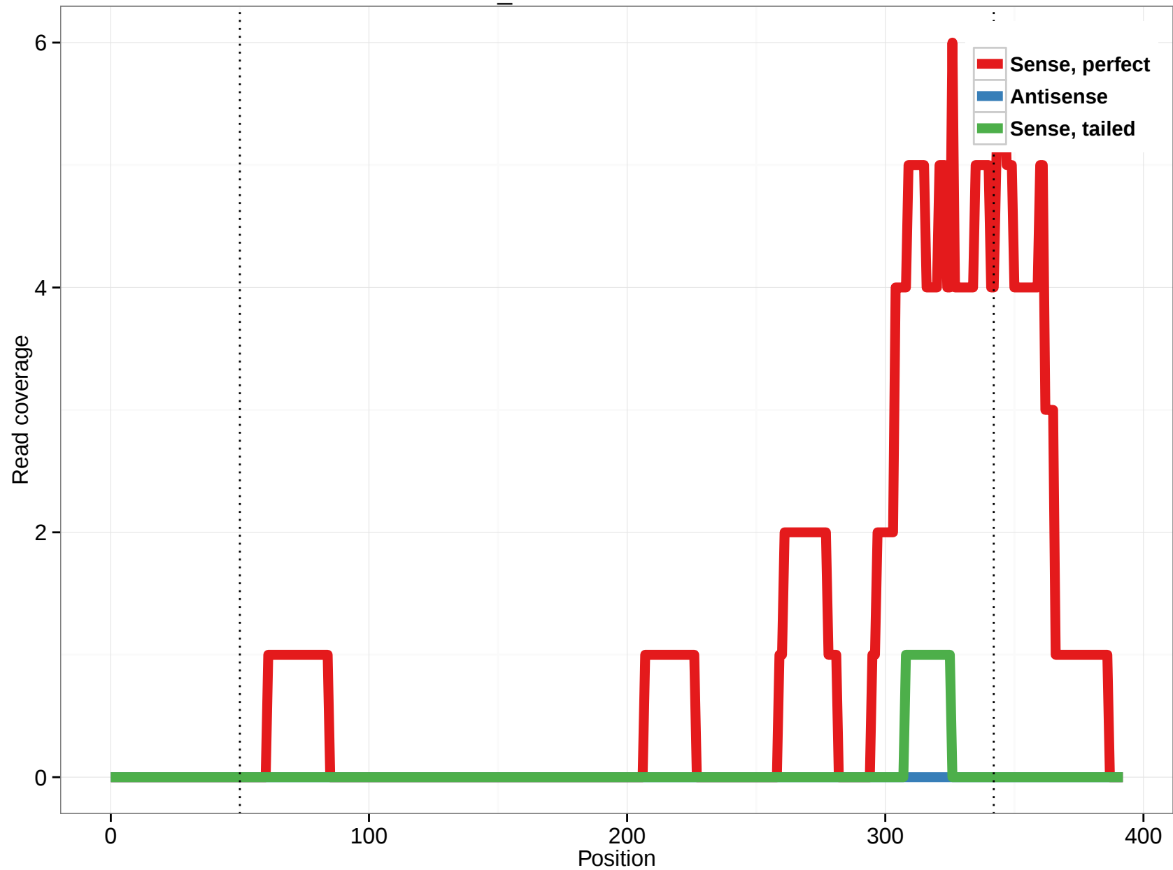
scaffold_4845:13831562-13831954
