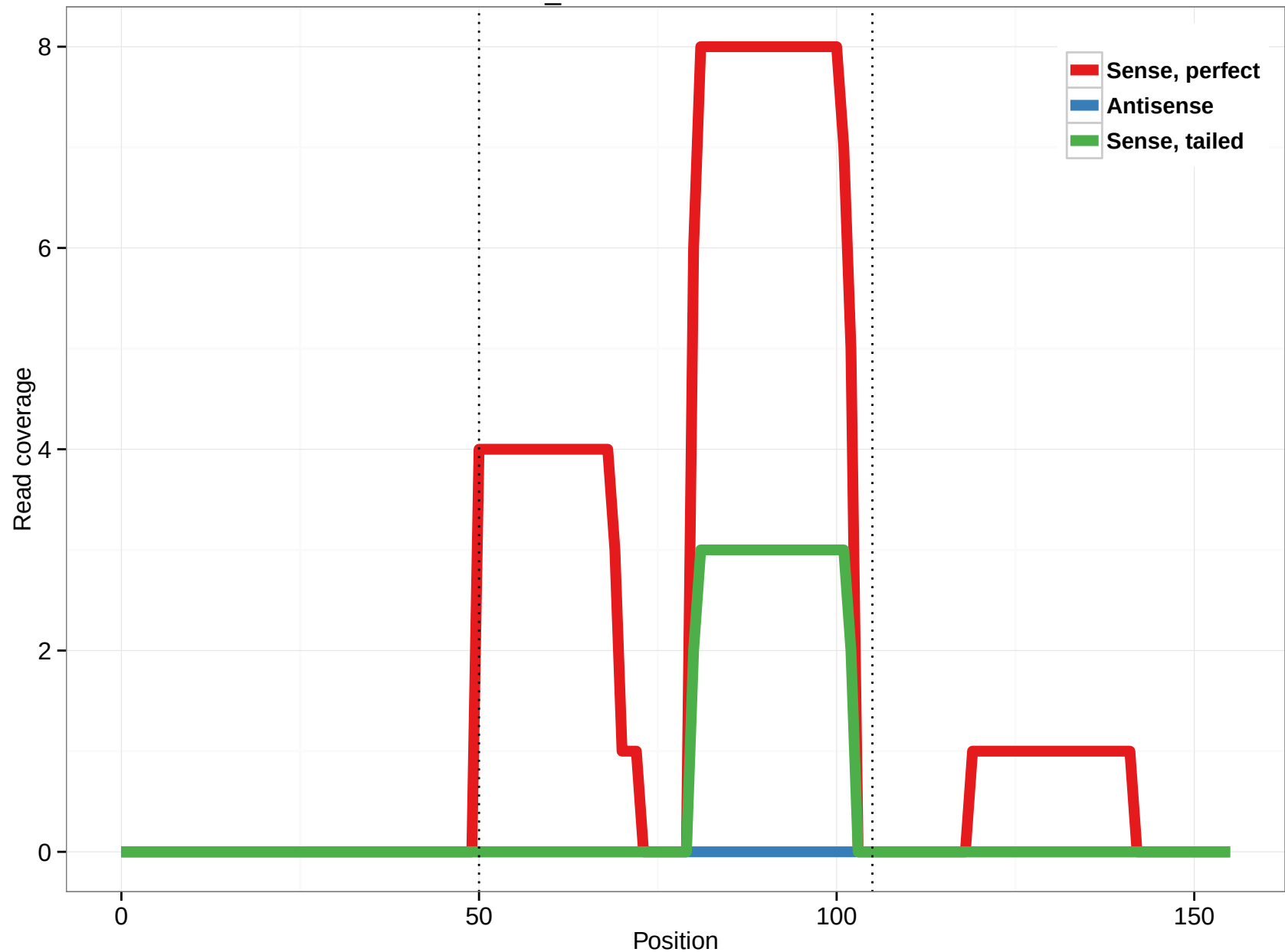
scaffold_4845:12896760-12896915
