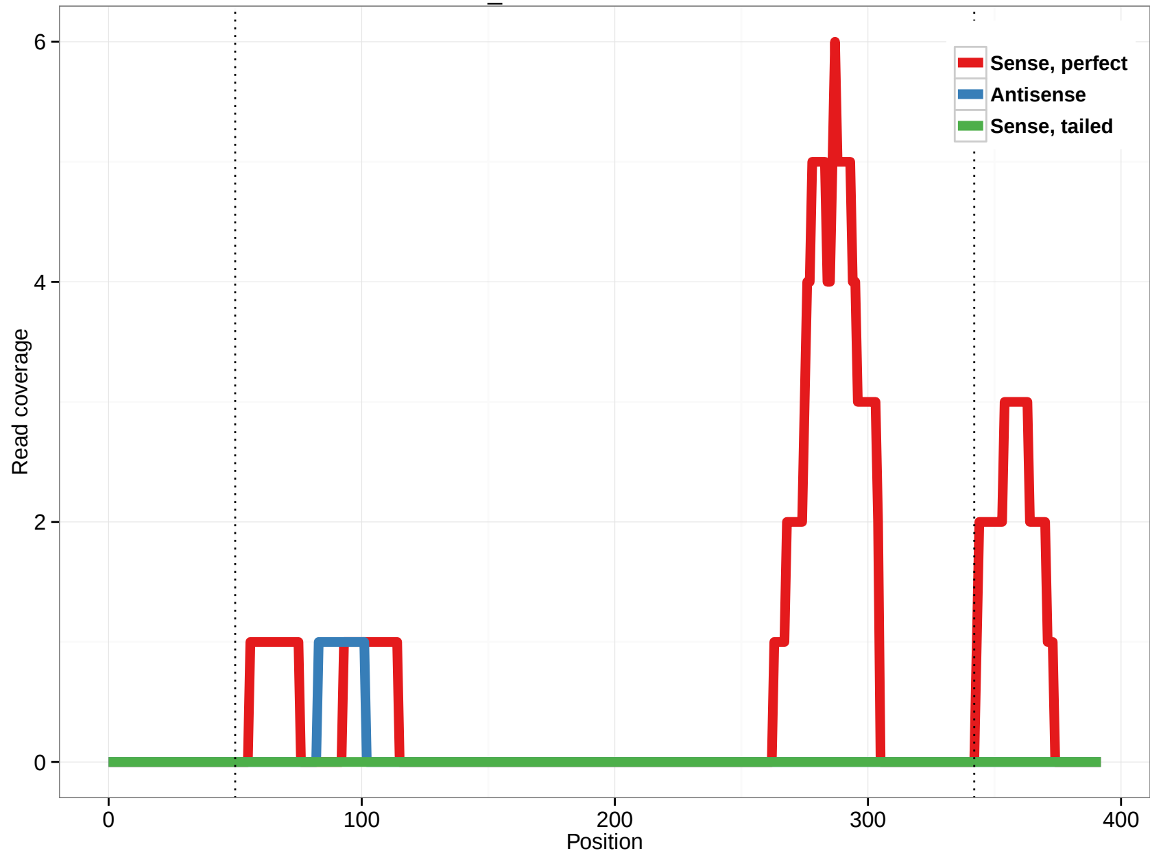
scaffold_4845:12863233-12863625
