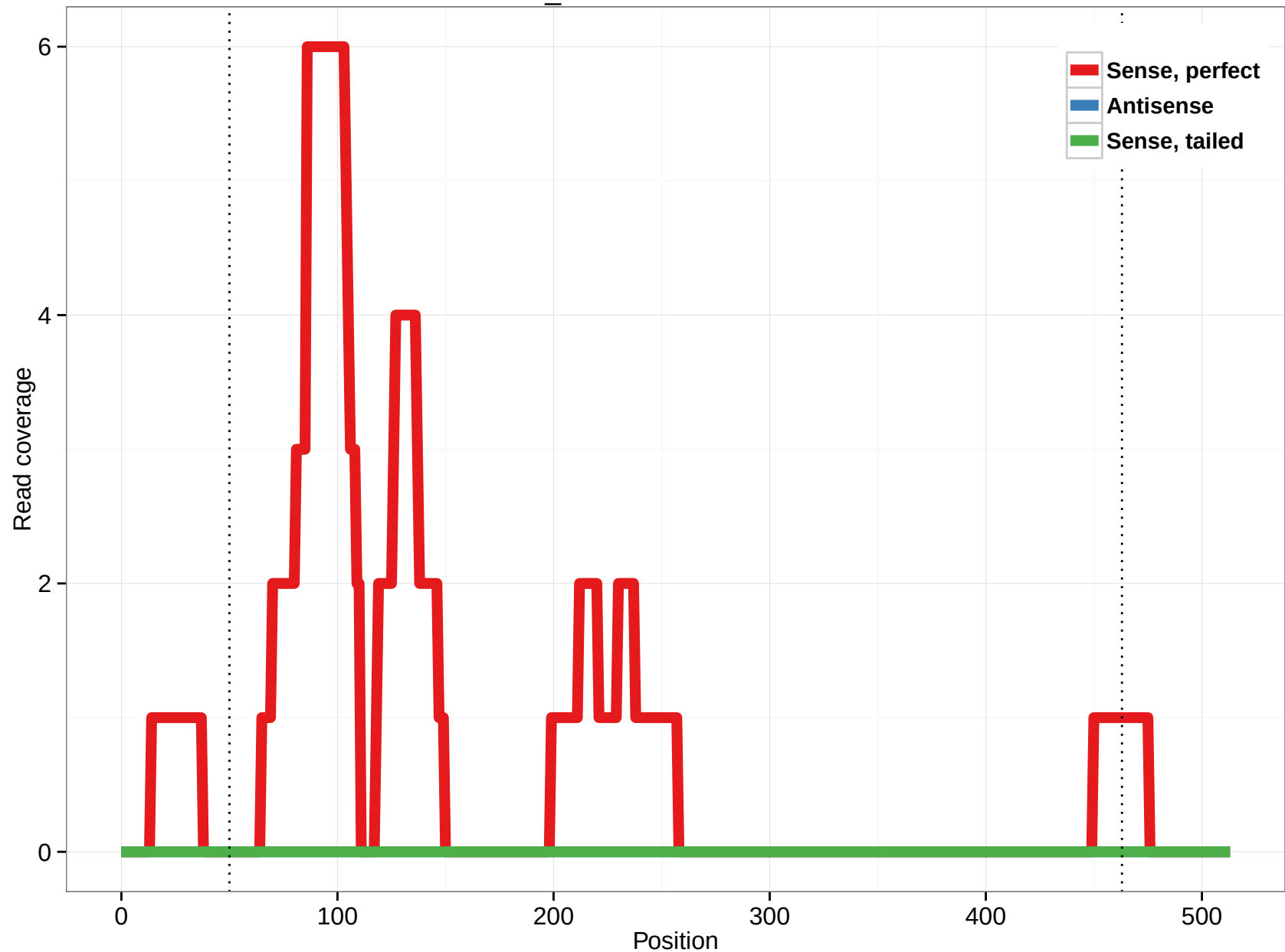
scaffold_4845:11701710-11702223
