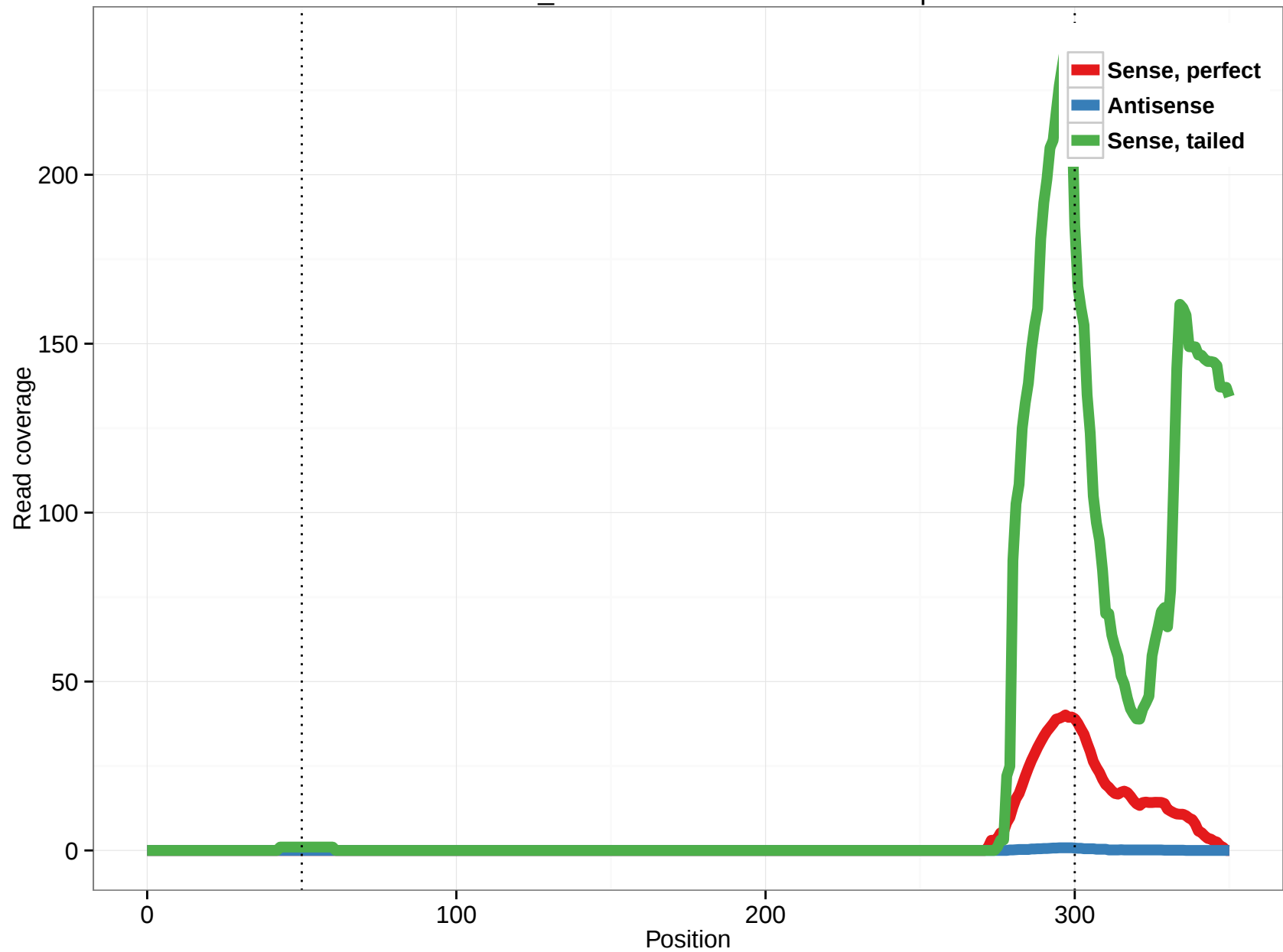
scaffold_4845:10270415-10271046.5p
