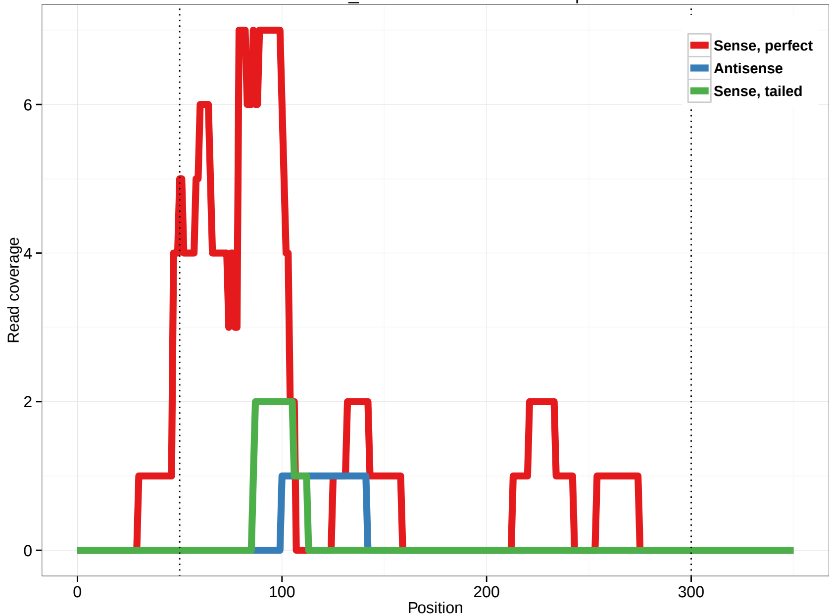
scaffold_4820:9894187-9895076.5p
