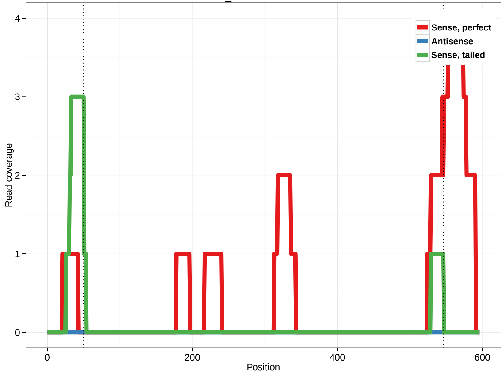
scaffold_4820:955716-956312
