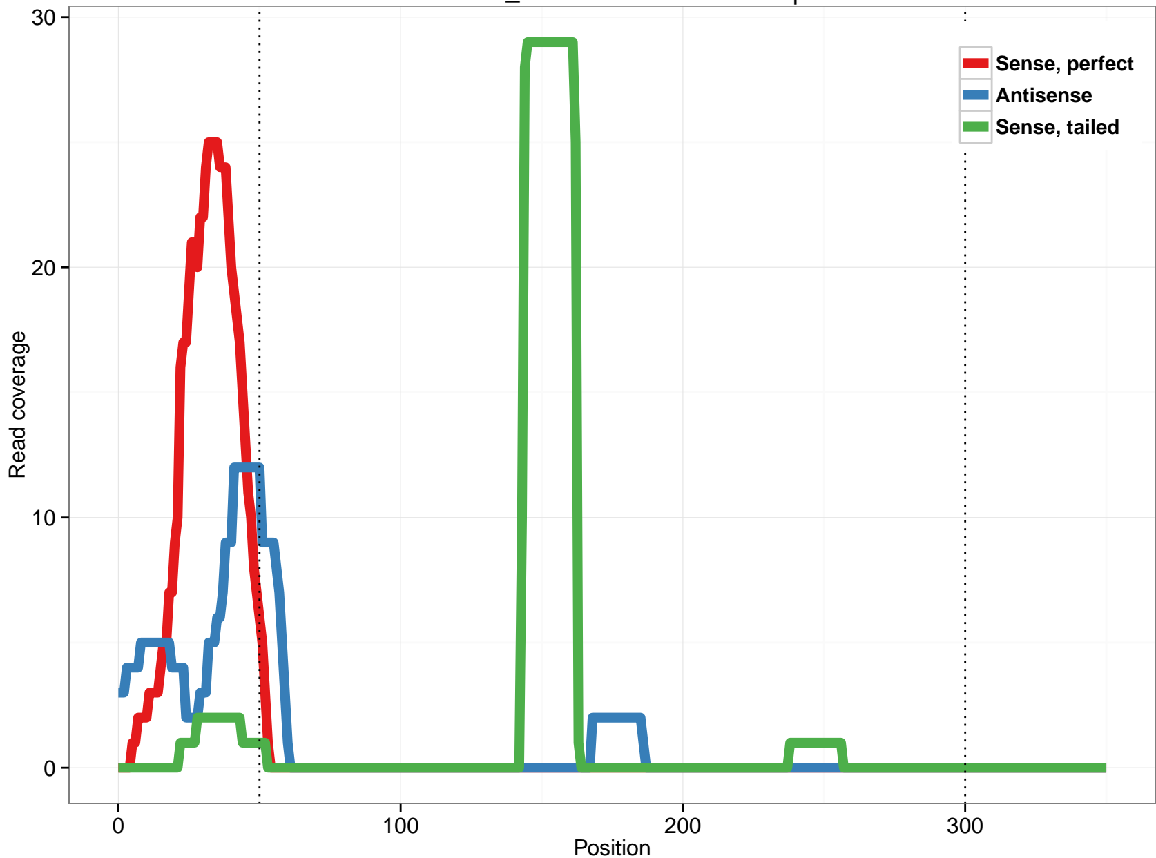
scaffold_4820:796635-798462.3p
