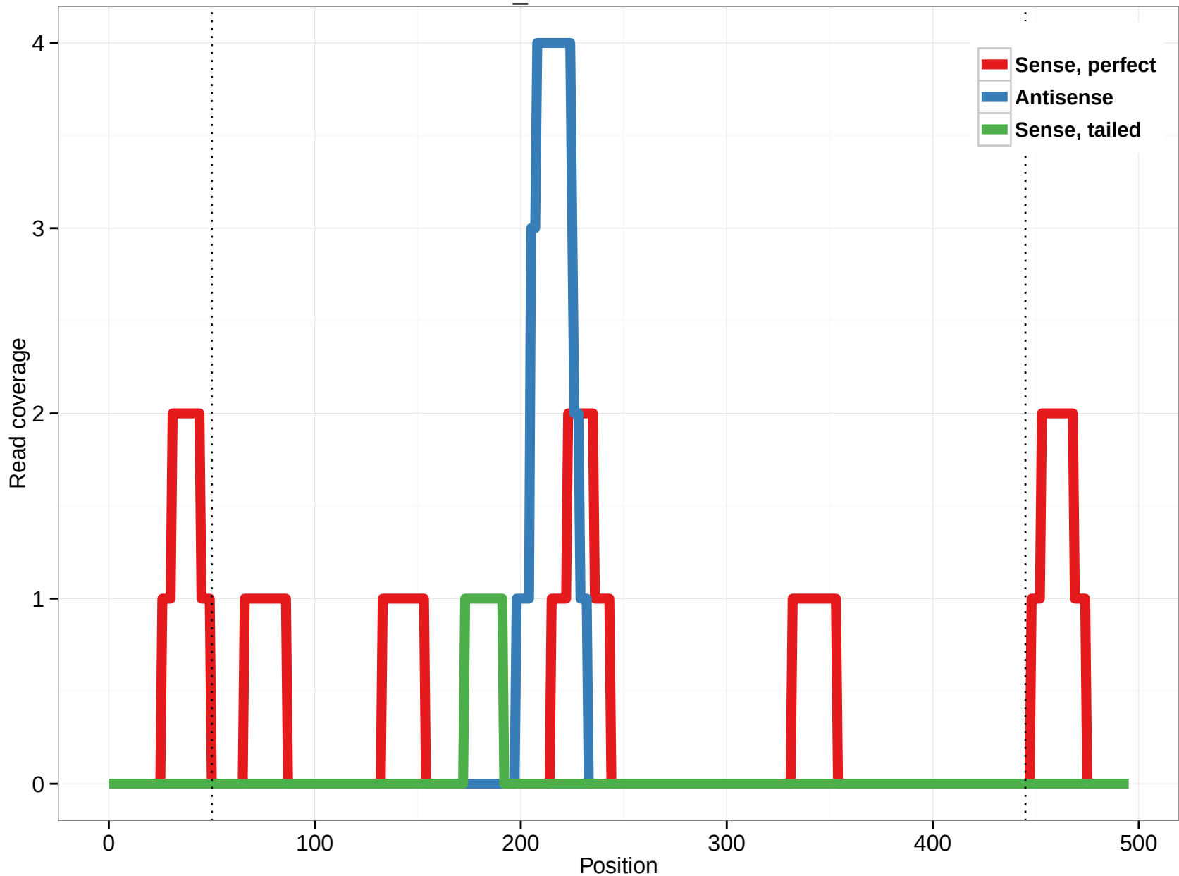
scaffold_4820:7914946-7915441
