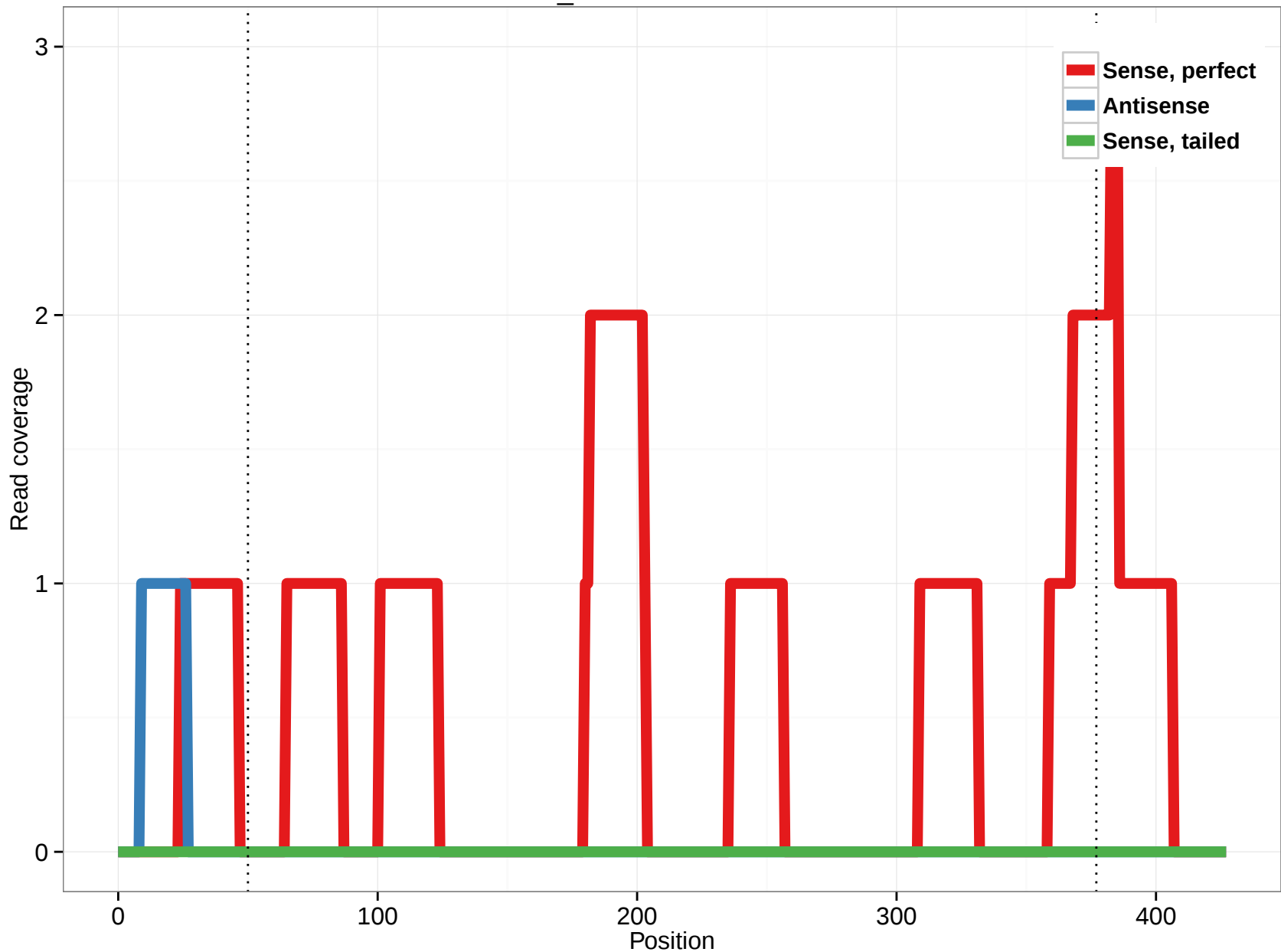
scaffold_4820:6994735-6995162
