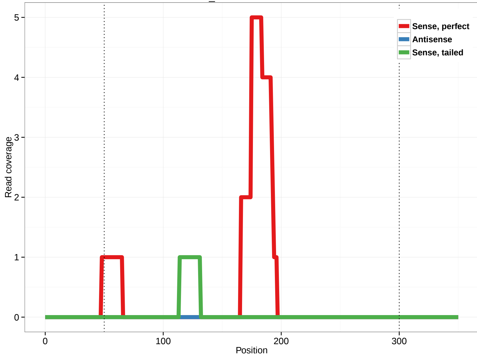
scaffold_4820:6569053-6569403
