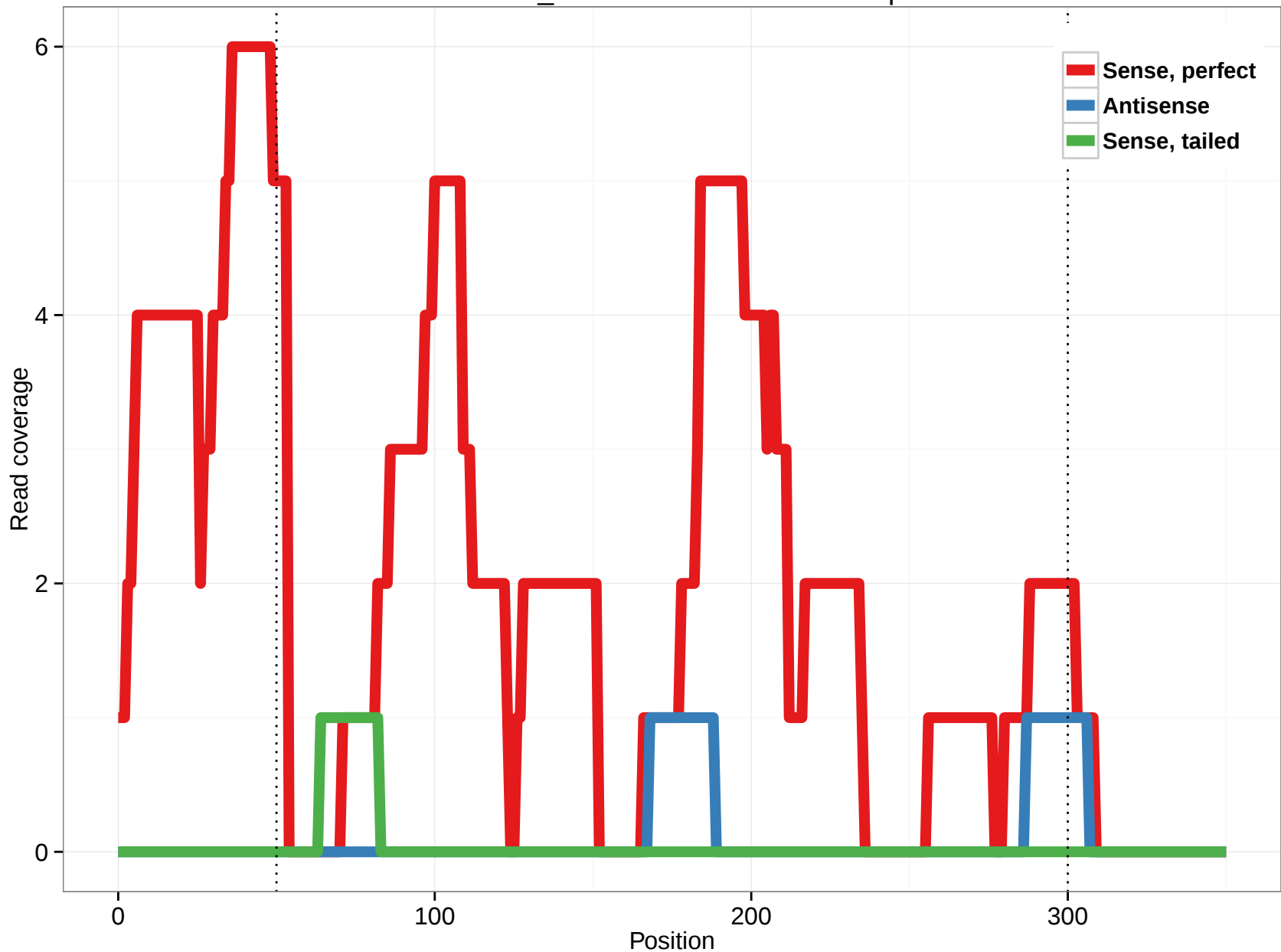
scaffold_4820:6533078-6533800.3p
