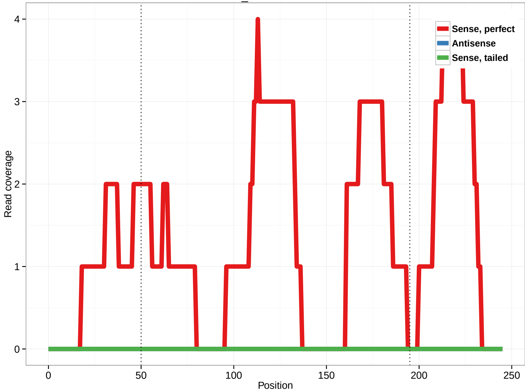
scaffold_4820:49735-49980
