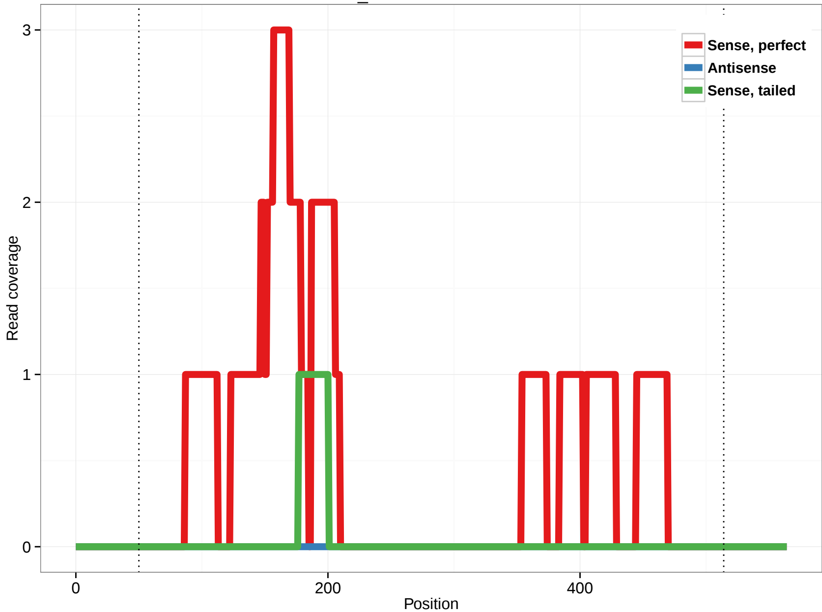
scaffold_4820:3098280-3098844
