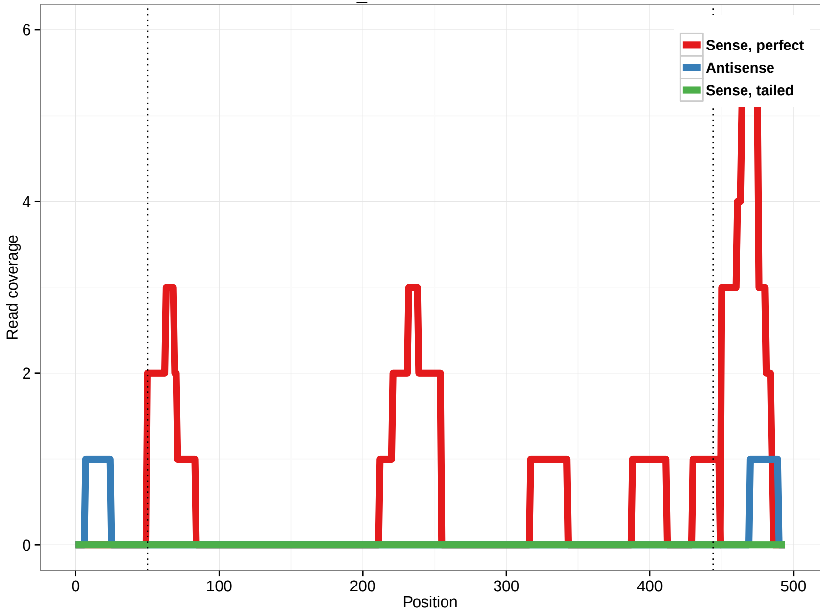
scaffold_4820:2434792-2435286
