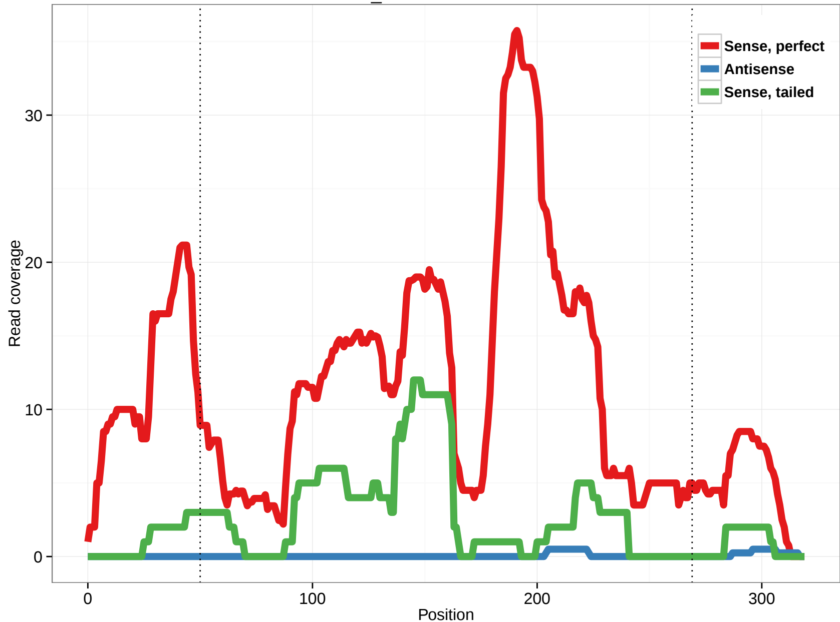
scaffold_4820:2260549-2260868
