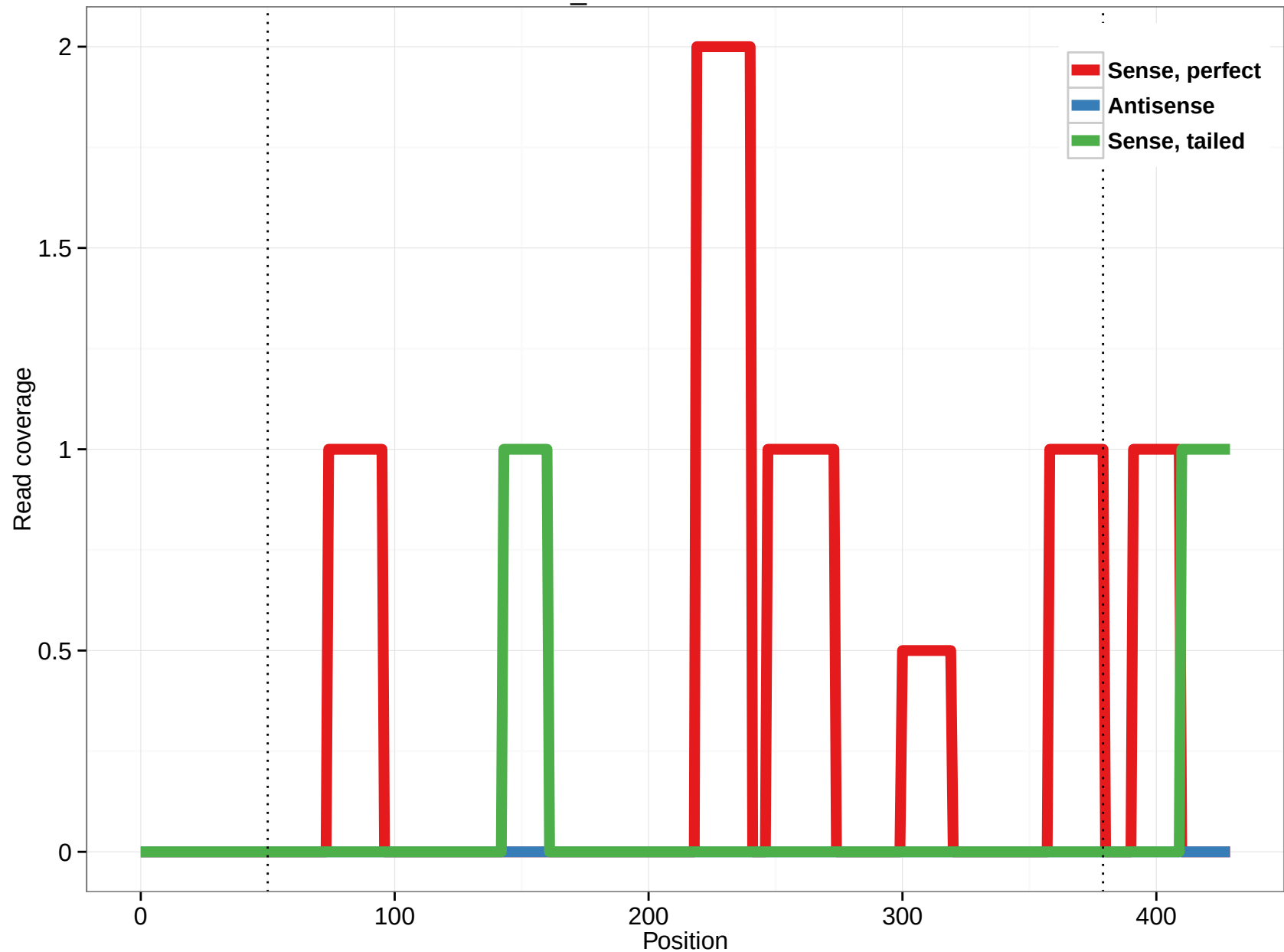
scaffold_4784:9744461-9744890
