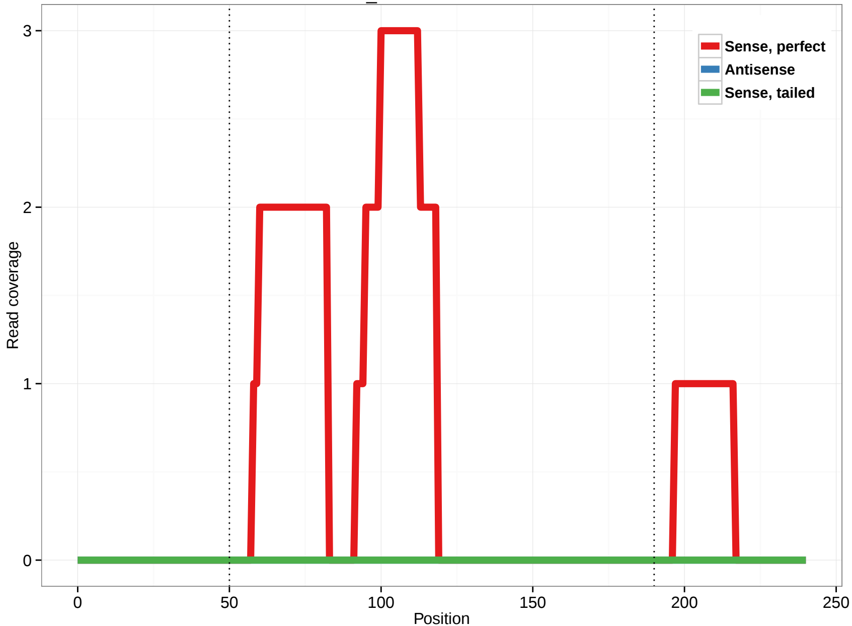
scaffold_4784:8497962-8498202
