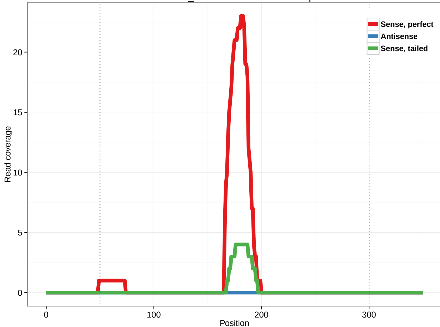
scaffold_4784:4036008-4036651.5p
