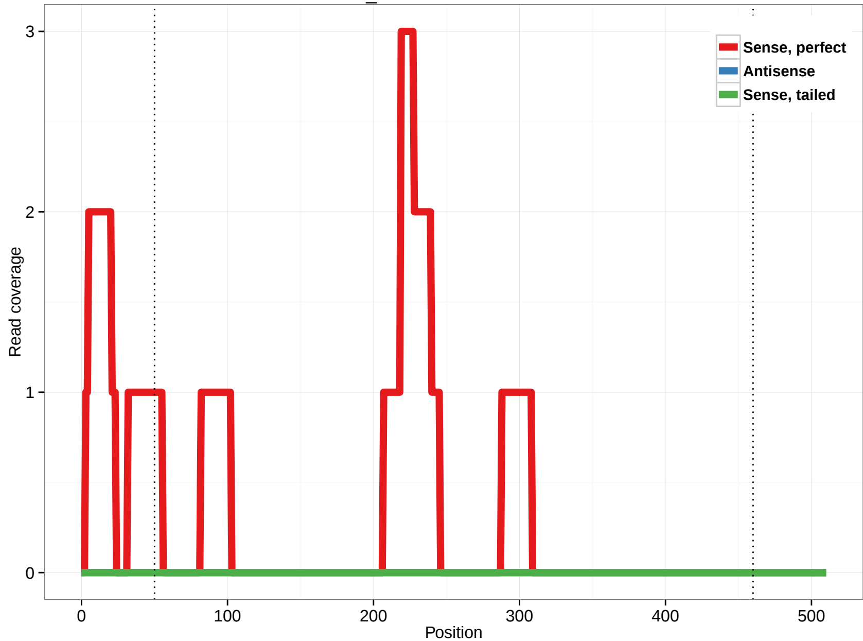
scaffold_4784:21629940-21630450
