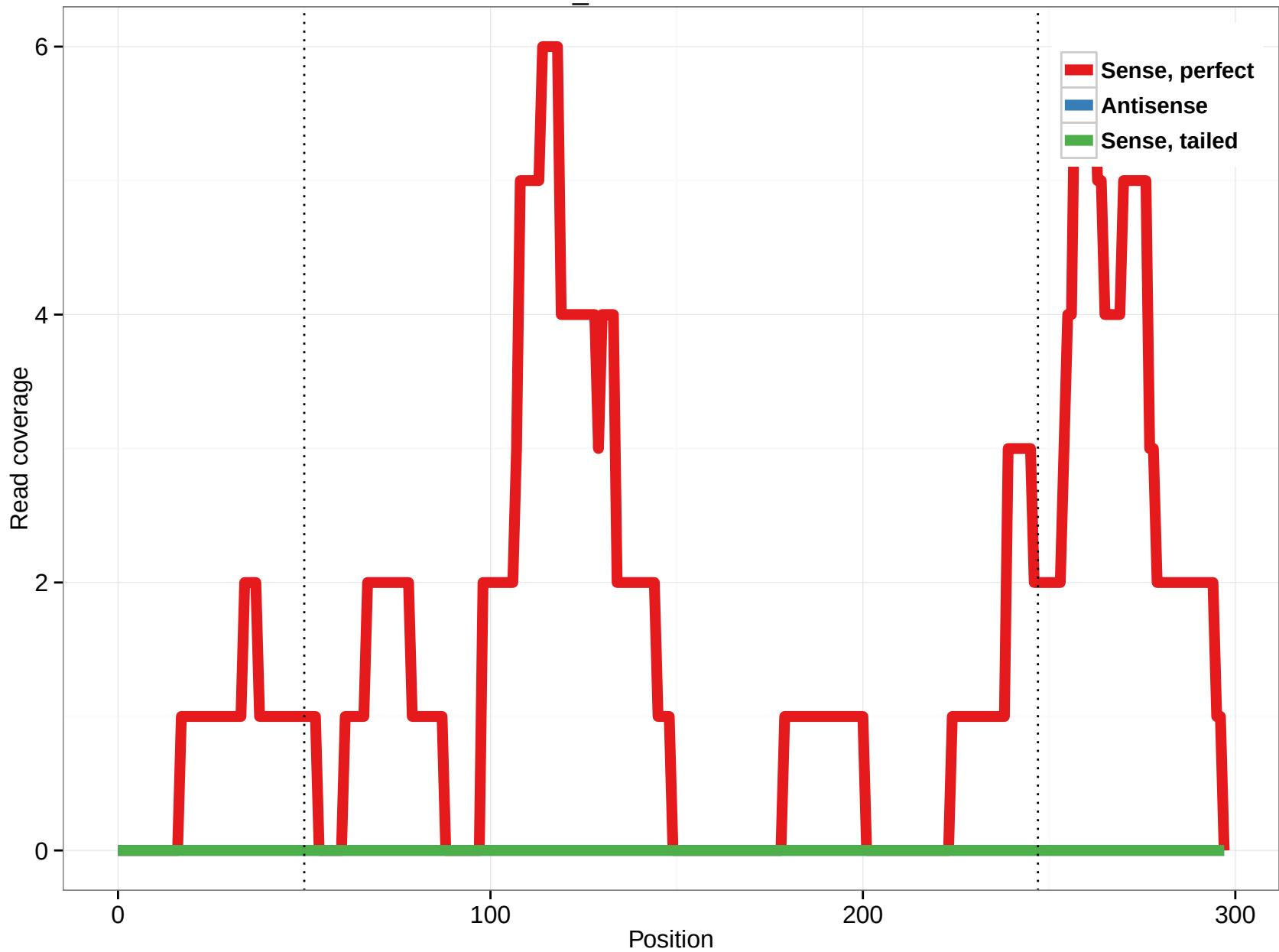
scaffold_4784:212933-213230
