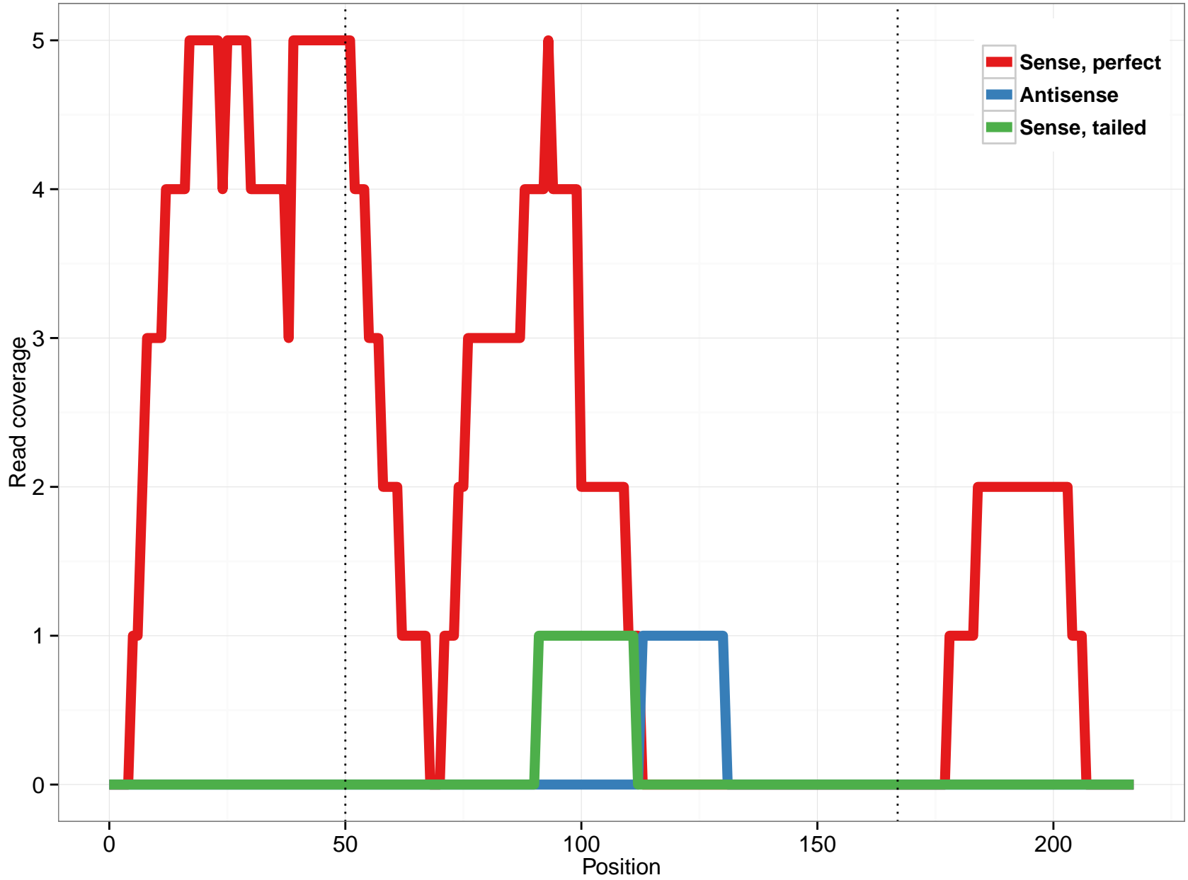
scaffold_4784:1536220-1536437
